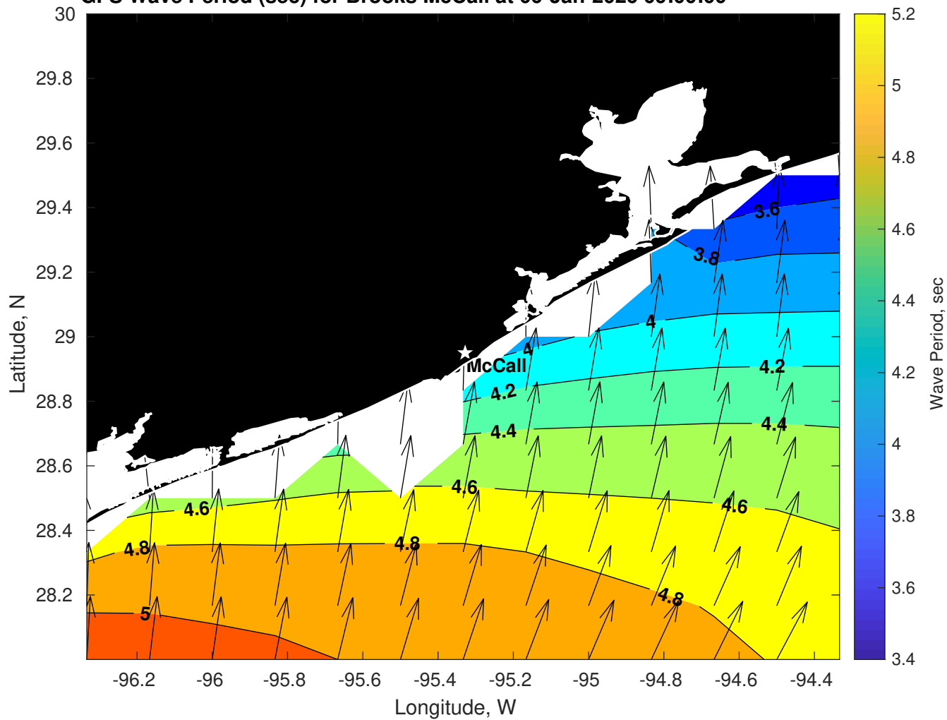
GFS Wave Period (sec) for Brooks McCall at 06-Jan-2026 09:00:00
