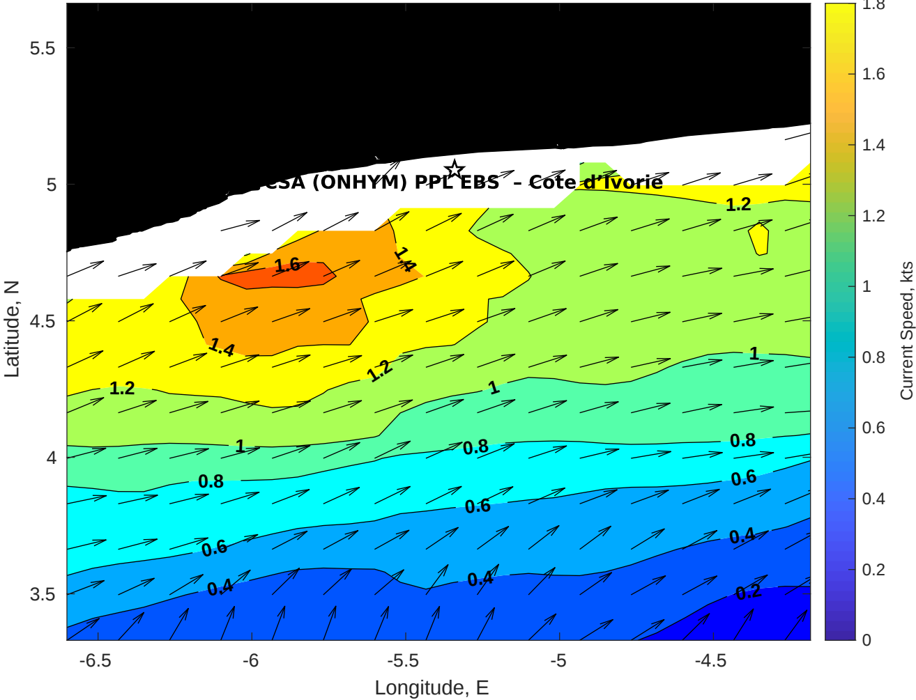
Surface Currents for CSA (ONHYM) PPL EBS - Cote d'Ivoire at 05-Jan-2026 00:00:00
