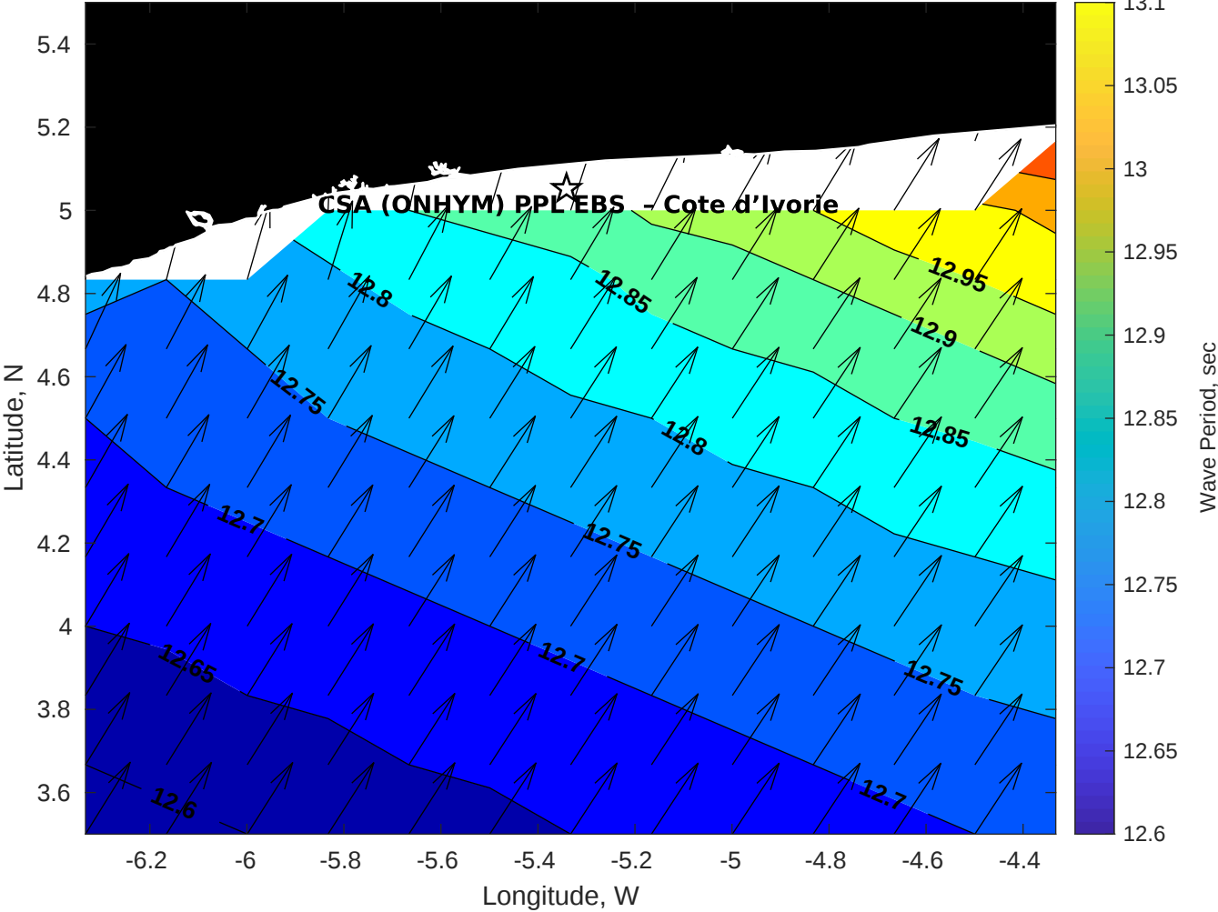
GFS Wave Period (sec) for CSA (ONHYM) PPL EBS - Cote d'Ivoire at 06-Jan-2026 09:00:00
