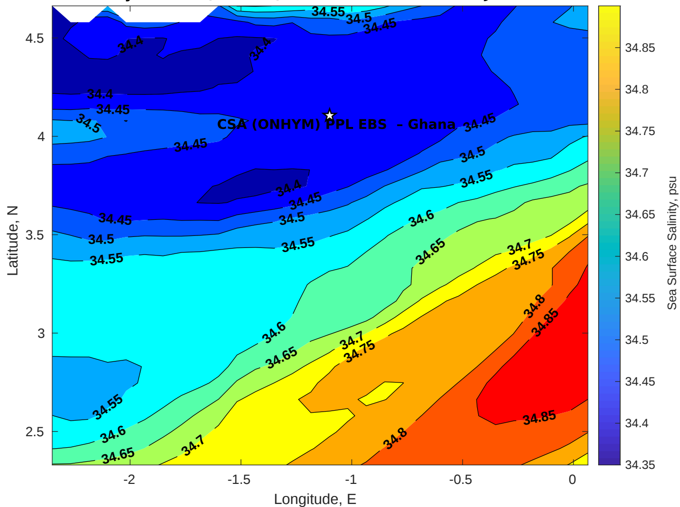
Surface Salinity for CSA (ONHYM) PPL EBS - Ghana at 05-Jan-2026 00:00:00
