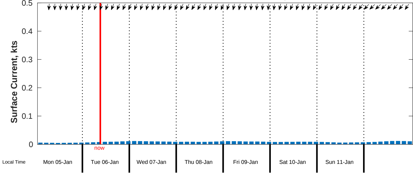
Surface Current Forecast for CSA (ONHYM) PPL EBS - Ghana from 05-Jan-2026 00:00:00 to 13-Jan-2026 00:00:00
