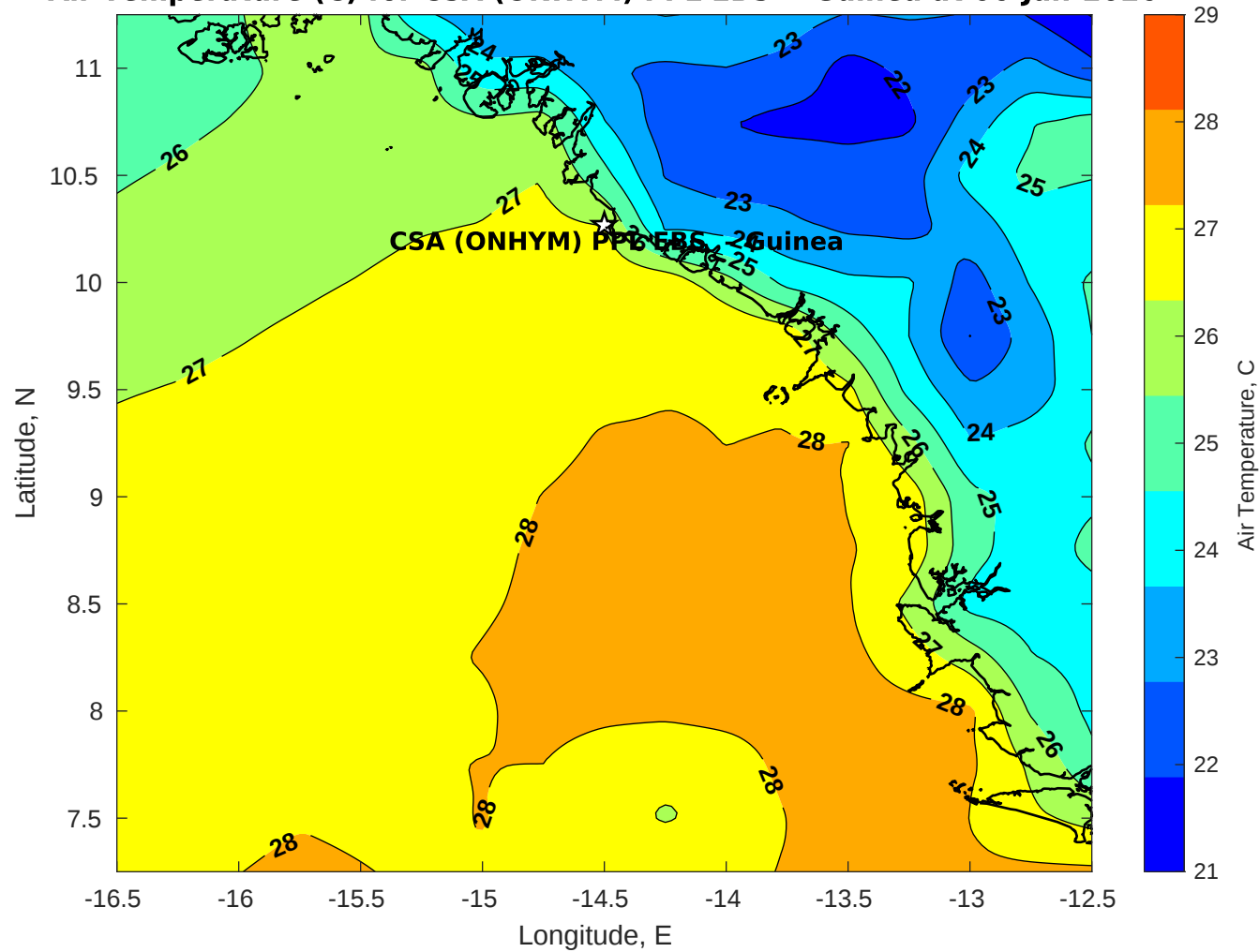
Air Temperature (C) for CSA (ONHYM) PPL EBS - Guinea at 06-Jan-2026
