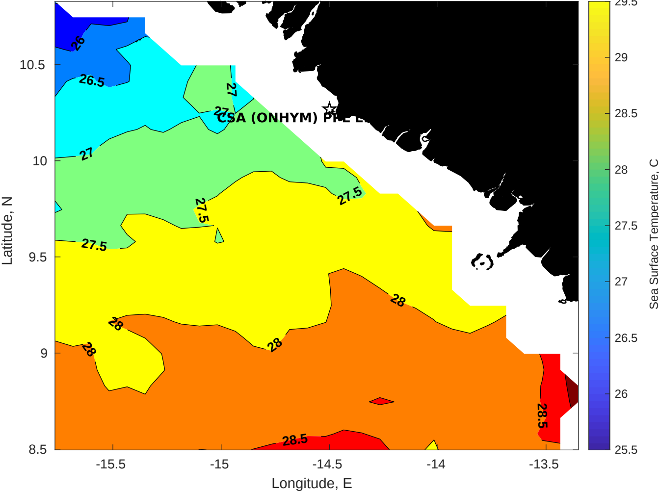
SST for CSA (ONHYM) PPL EBS - Guinea at 05-Jan-2026 00:00:00
