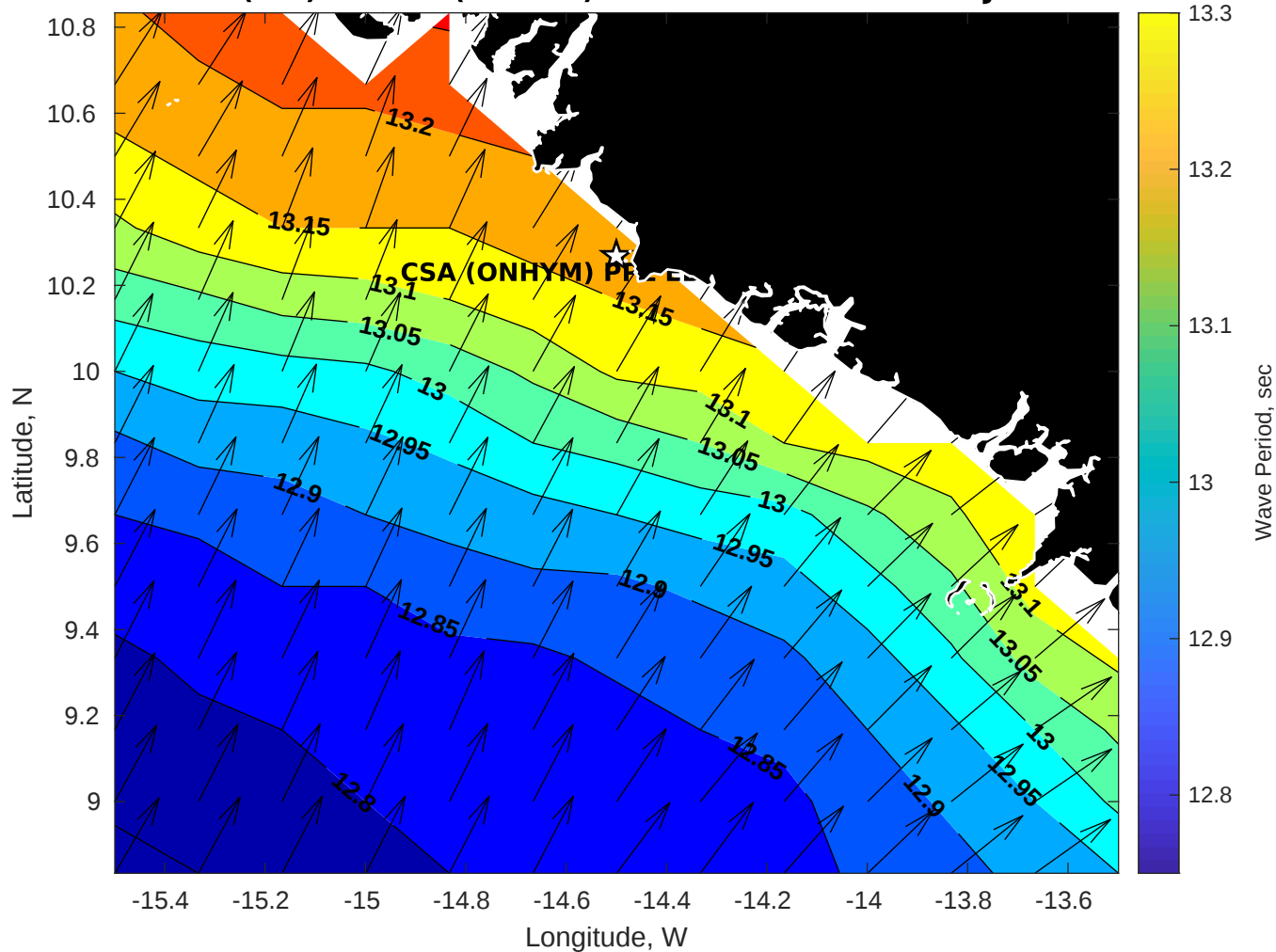
GFS Wave Period (sec) for CSA (ONHYM) PPL EBS - Guinea at 06-Jan-2026 09:00:00
