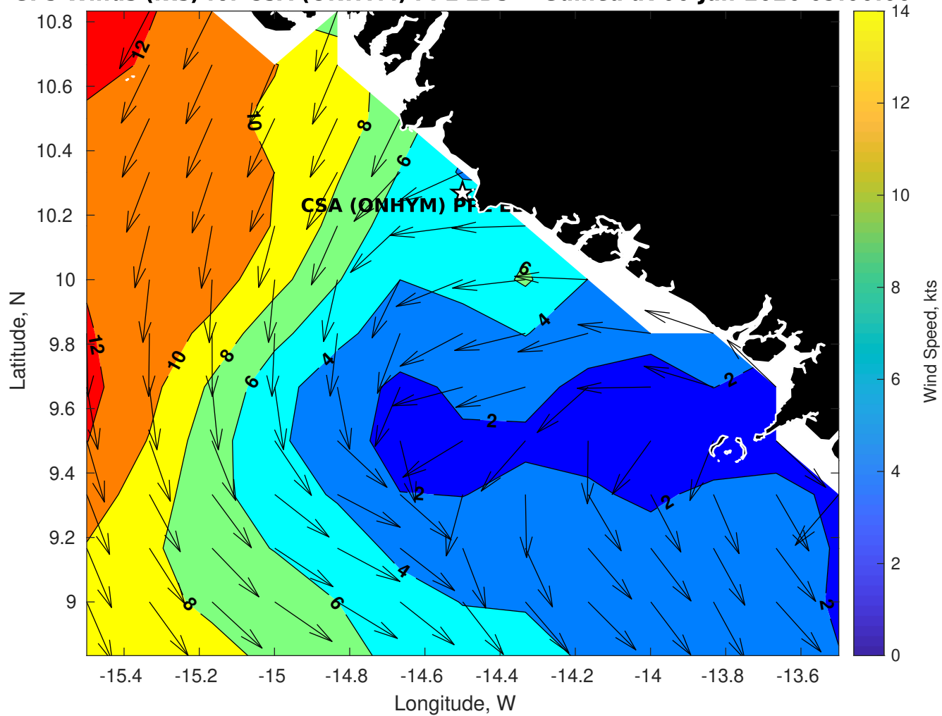
GFS Winds (kts) for CSA (ONHYM) PPL EBS - Guinea at 06-Jan-2026 09:00:00
