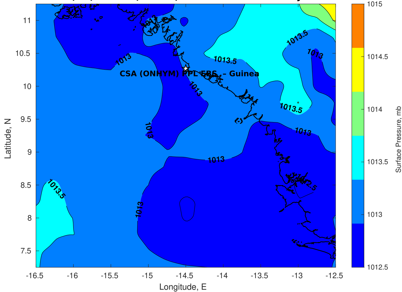
Surface Pressure (mb) for CSA (ONHYM) PPL EBS - Guinea at 06-Jan-2026 00:00:00
