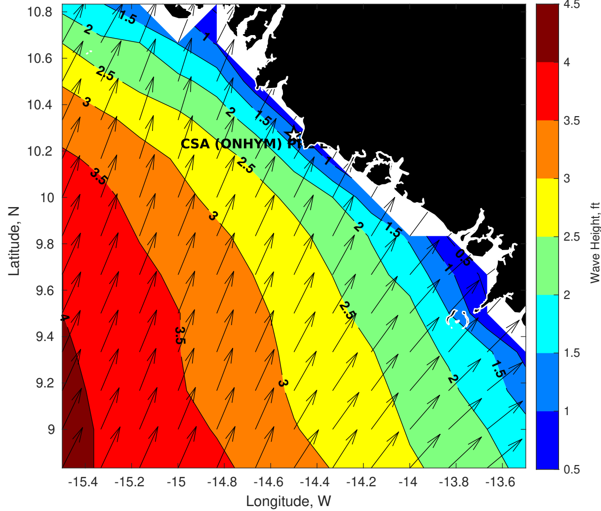
GFS Wave Height (ft) for CSA (ONHYM) PPL EBS - Guinea at 06-Jan-2026 09:00:00
