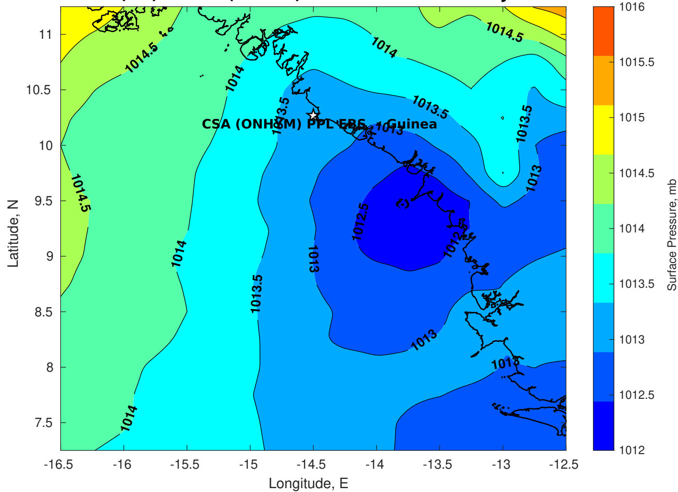
Surface Pressure (mb) for CSA (ONHYM) PPL EBS - Guinea at 08-Jan-2026 00:00:00
