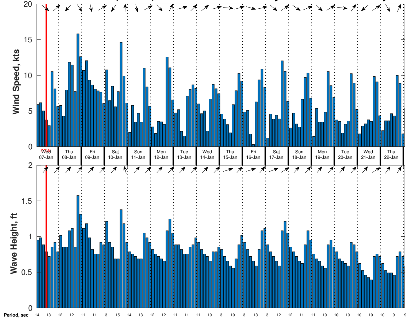
Wind & Wave Forecast for CSA (ONHYM) PPL EBS - Guinea from 06-Jan-2026 01:00:00 to 22-Jan-2026 01:00:00
