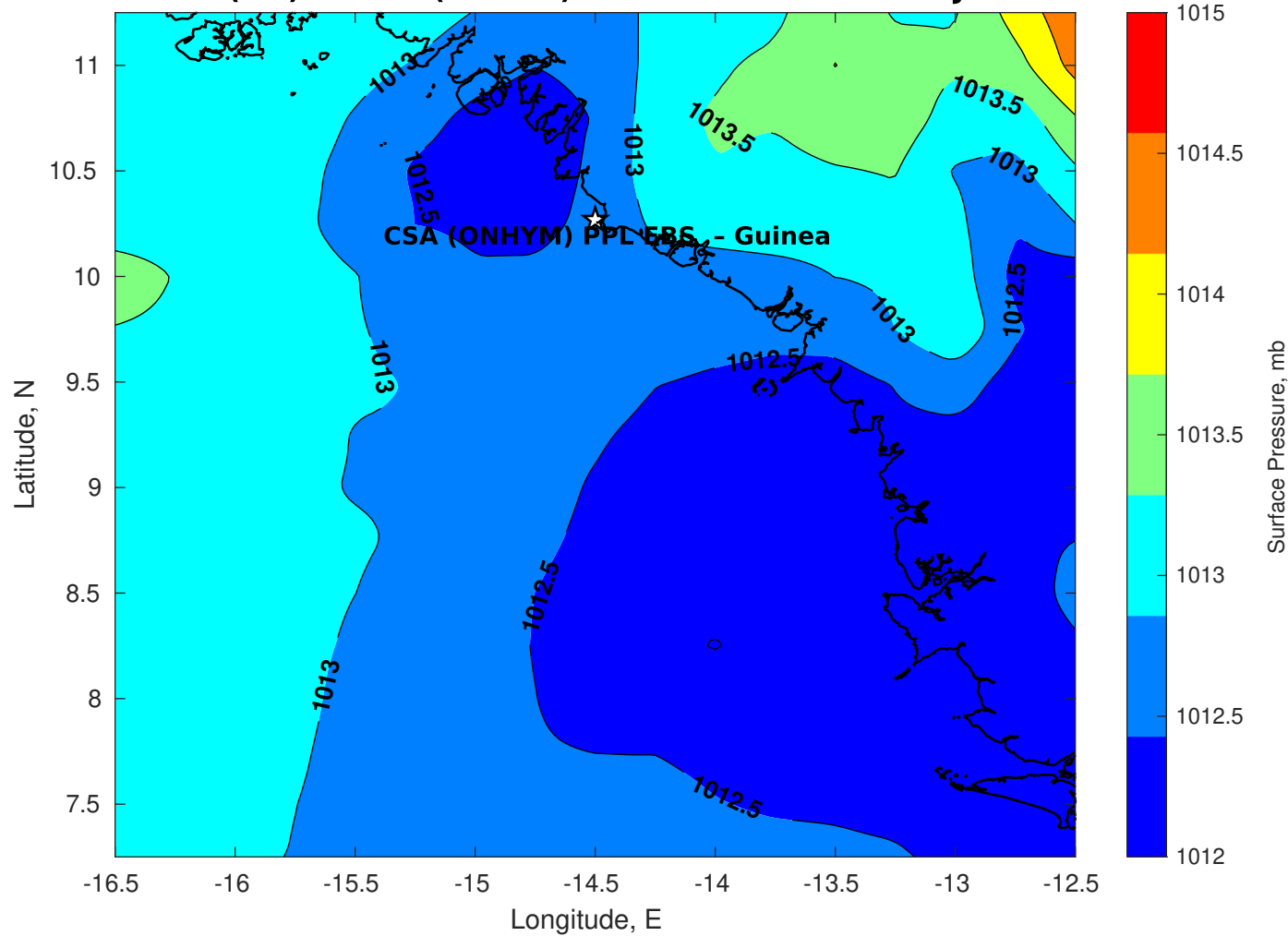
Surface Pressure (mb) for CSA (ONHYM) PPL EBS - Guinea at 07-Jan-2026 00:00:00
