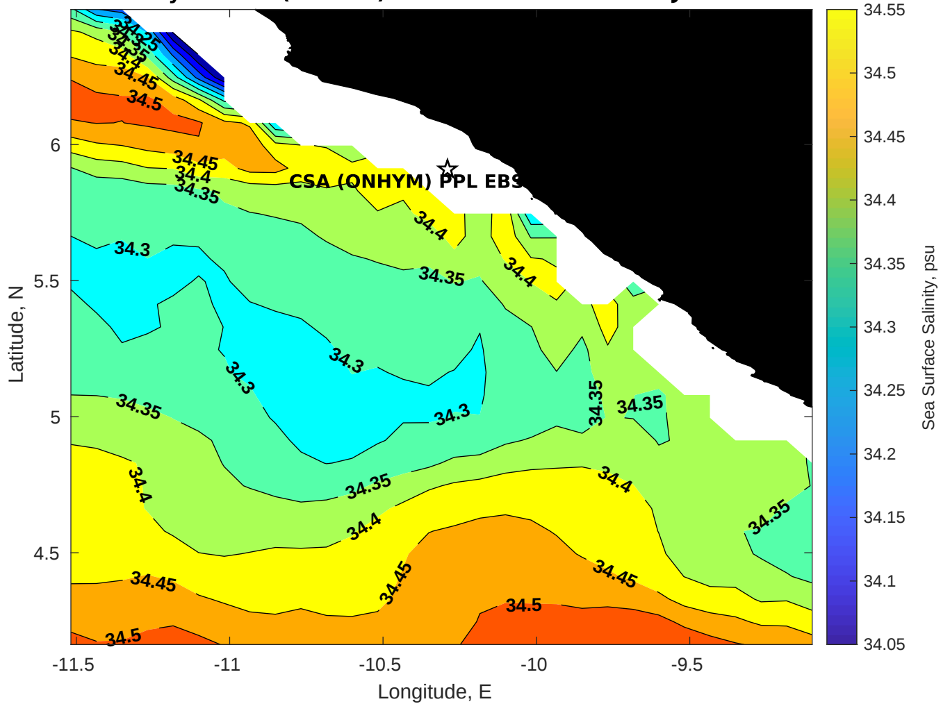
Surface Salinity for CSA (ONHYM) PPL EBS - Liberia at 05-Jan-2026 00:00:00
