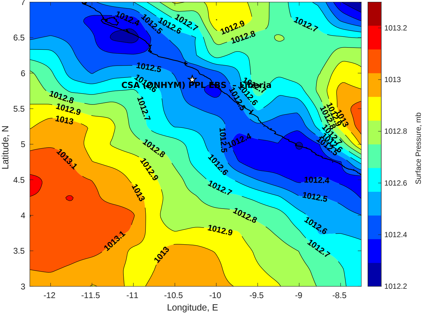
Surface Pressure (mb) for CSA (ONHYM) PPL EBS - Liberia at 07-Jan-2026 00:00:00
