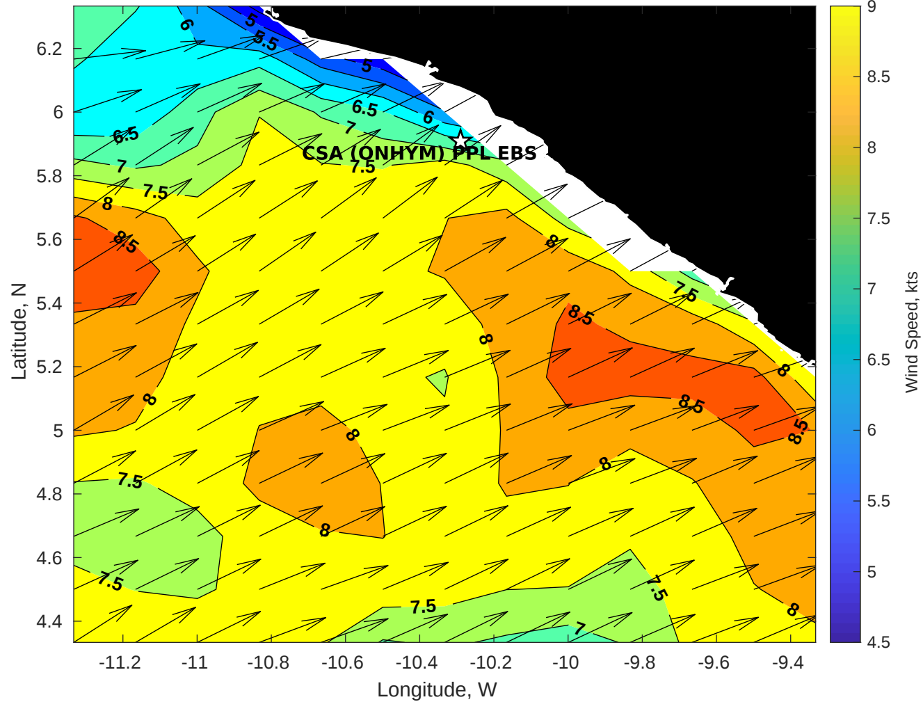
GFS Winds (kts) for CSA (ONHYM) PPL EBS - Liberia at 06-Jan-2026 09:00:00
