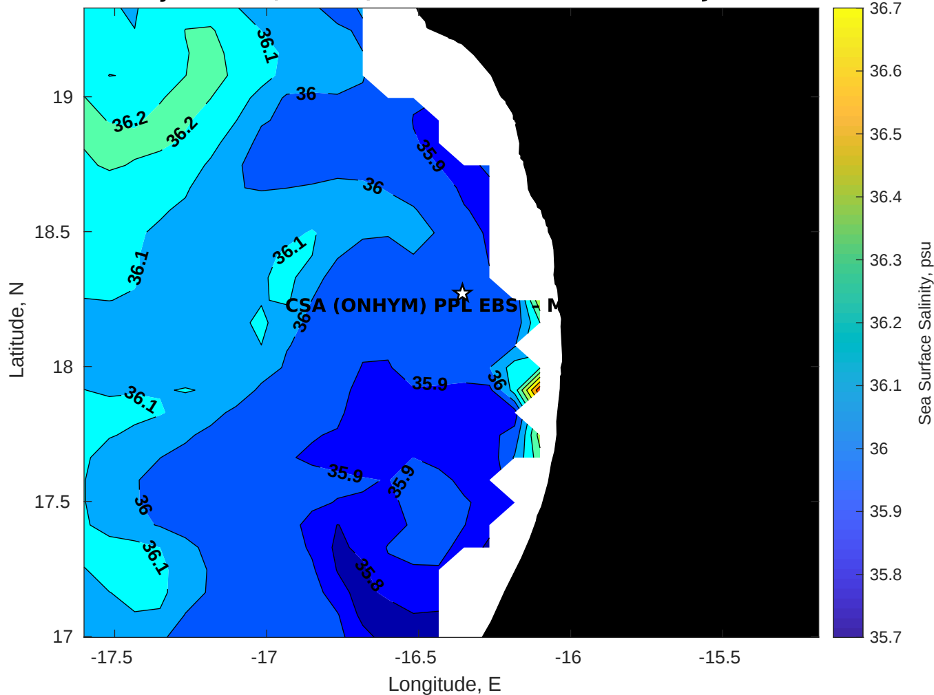
Surface Salinity for CSA (ONHYM) PPL EBS - Mauritania at 05-Jan-2026 00:00:00
