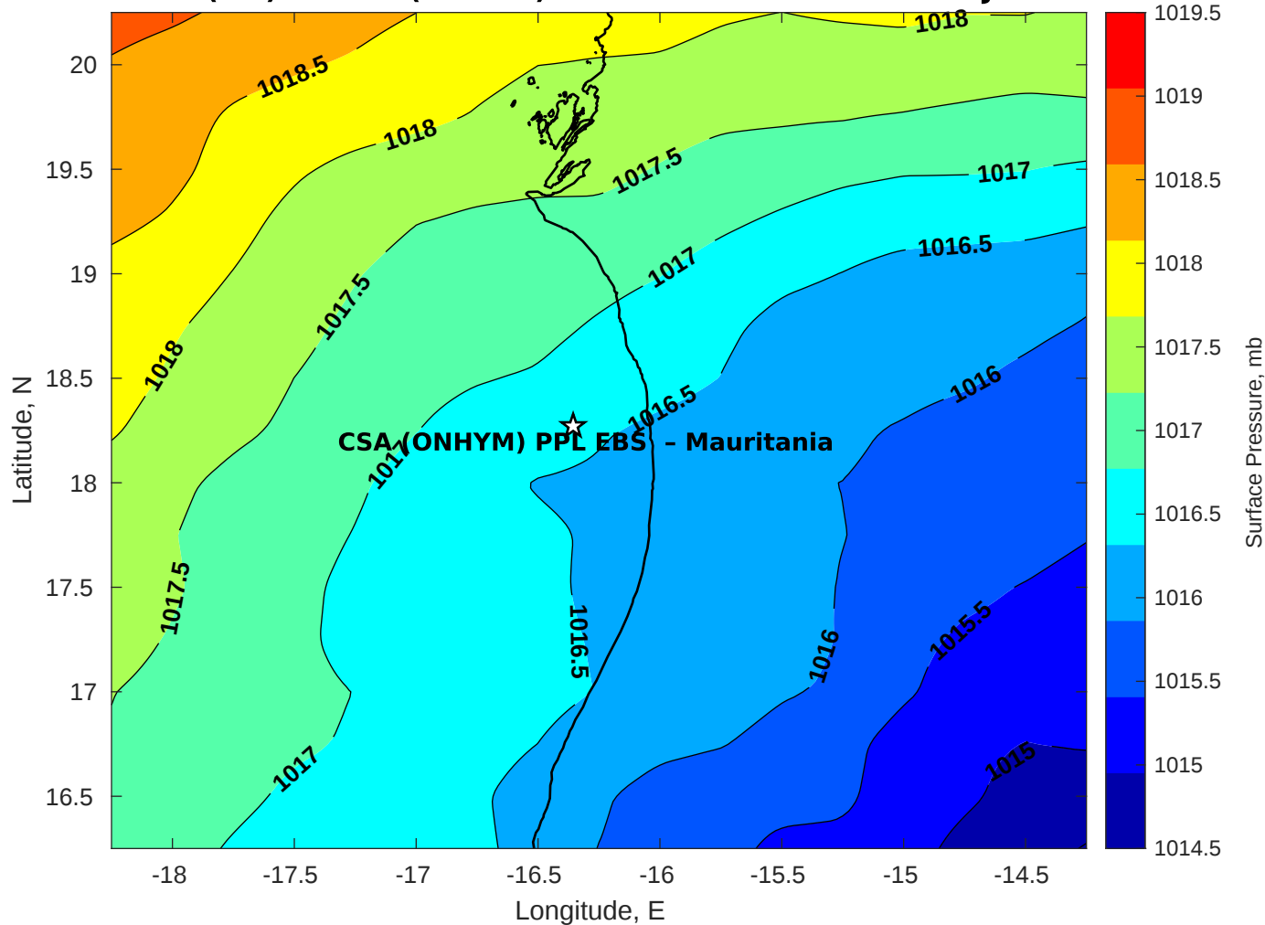
Surface Pressure (mb) for CSA (ONHYM) PPL EBS - Mauritania at 07-Jan-2026 00:00:00
