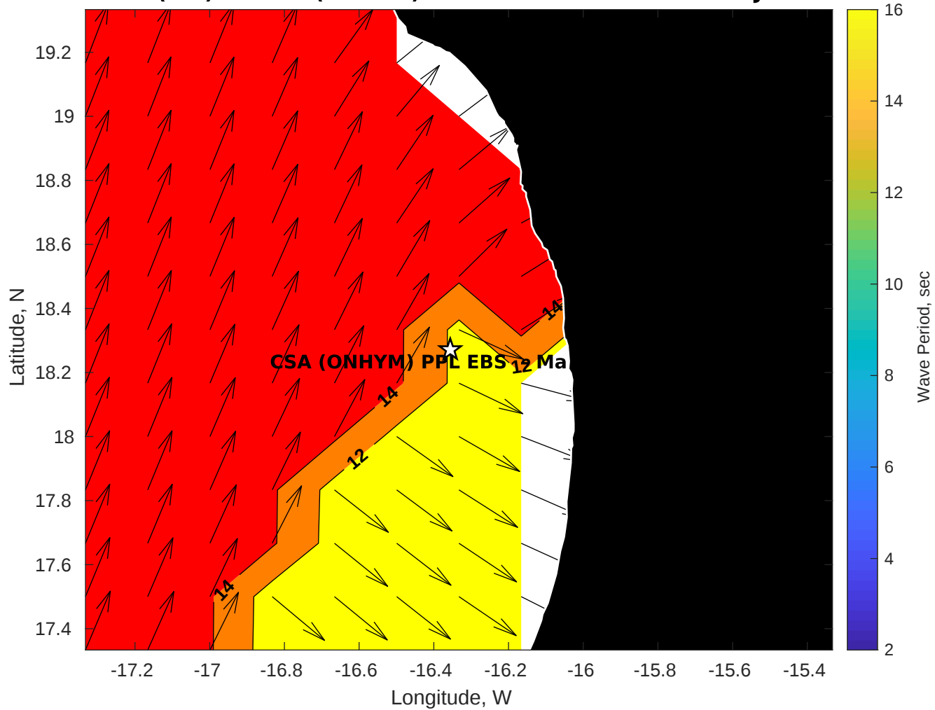
GFS Wave Period (sec) for CSA (ONHYM) PPL EBS - Mauritania at 06-Jan-2026 09:00:00
