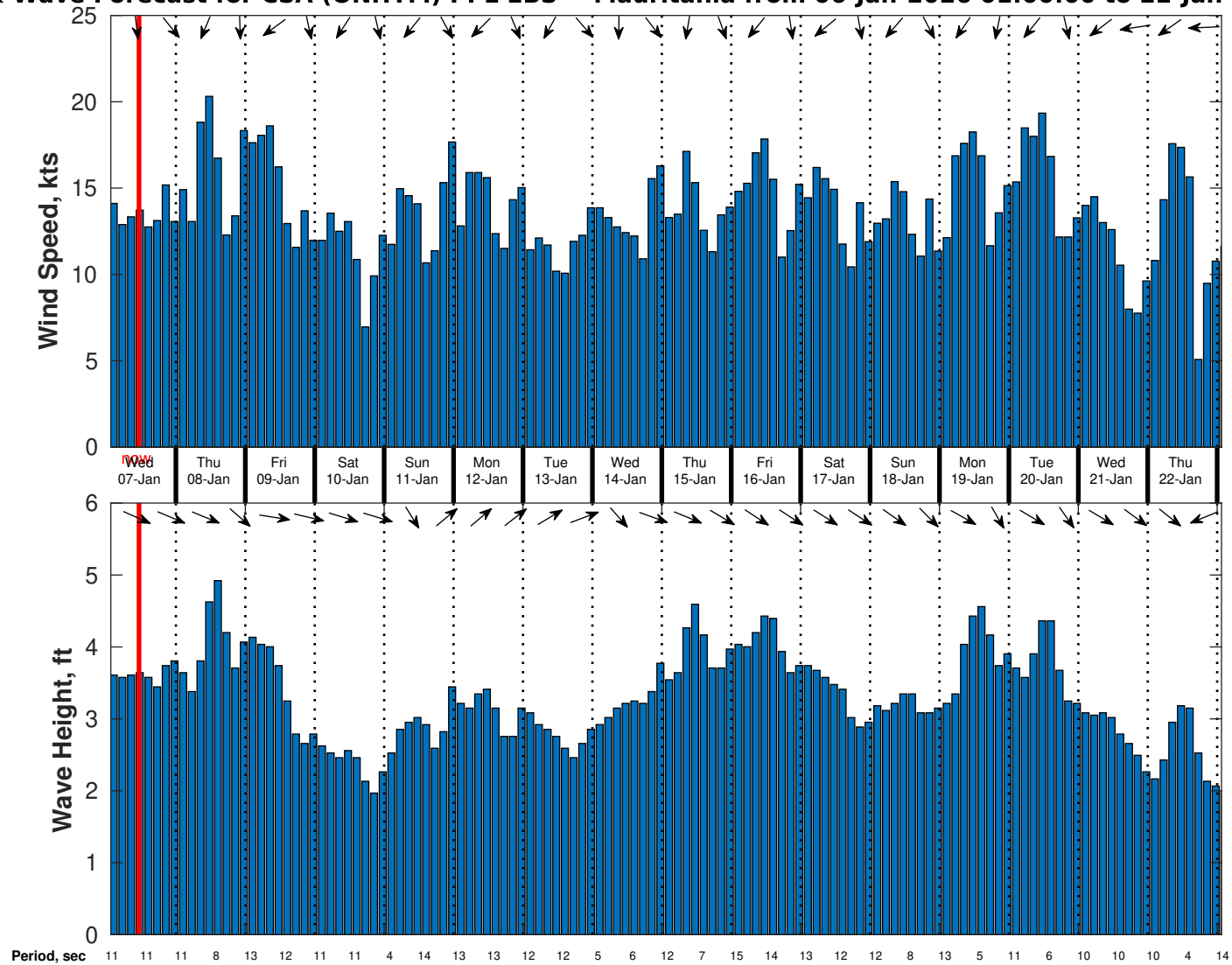
Wind & Wave Forecast for CSA (ONHYM) PPL EBS - Mauritania from 06-Jan-2026 01:00:00 to 22-Jan-2026 01:00:00
