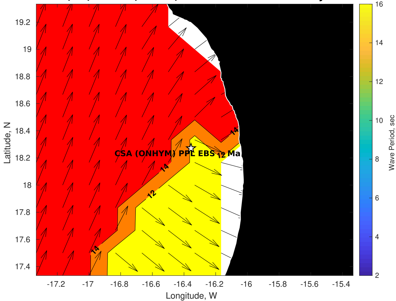
GFS Wave Period (sec) for CSA (ONHYM) PPL EBS - Mauritania at 06-Jan-2026 09:00:00
