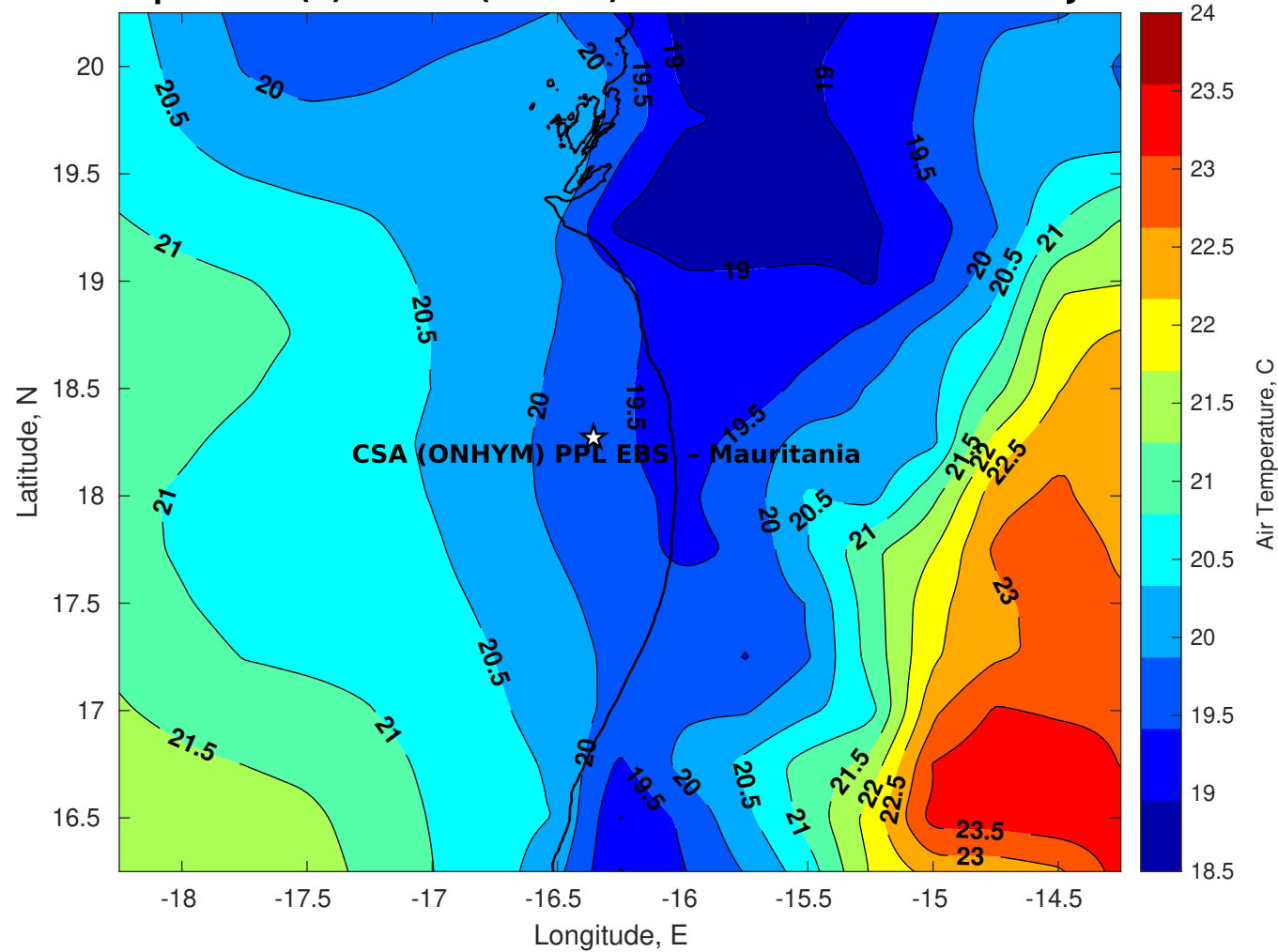
Air Temperature (C) for CSA (ONHYM) PPL EBS - Mauritania at 06-Jan-2026
