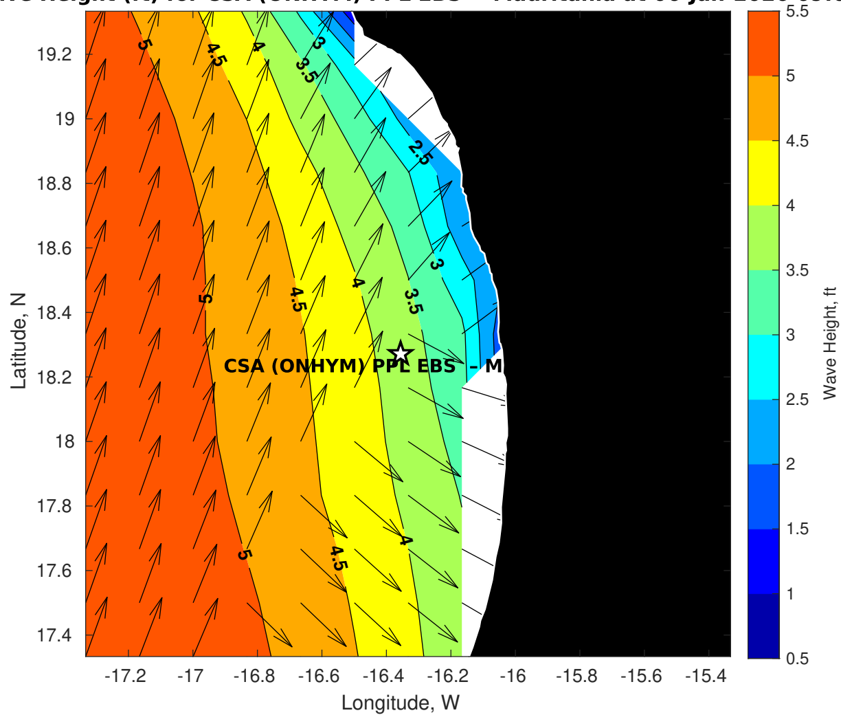
GFS Wave Height (ft) for CSA (ONHYM) PPL EBS - Mauritania at 06-Jan-2026 09:00:00
