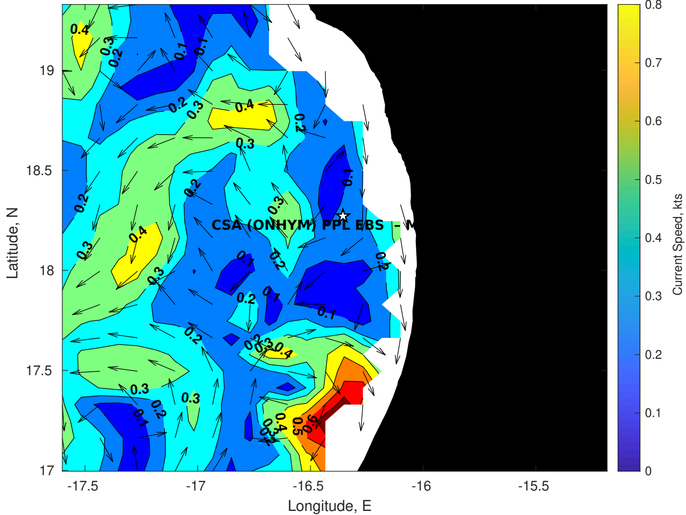
Surface Currents for CSA (ONHYM) PPL EBS - Mauritania at 05-Jan-2026 00:00:00
