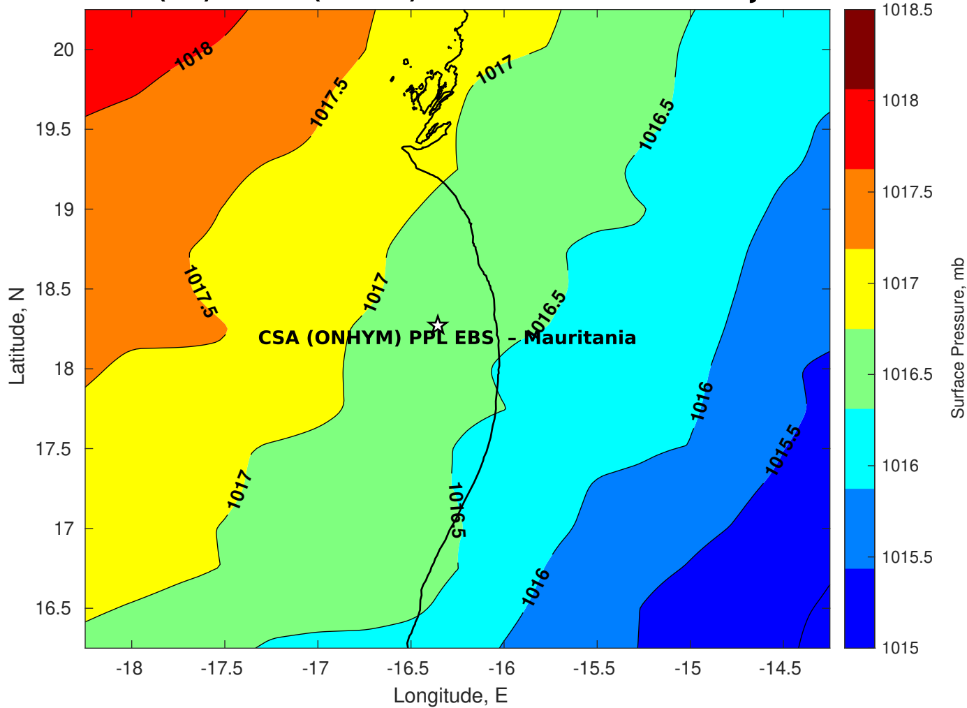
Surface Pressure (mb) for CSA (ONHYM) PPL EBS - Mauritania at 06-Jan-2026 00:00:00
