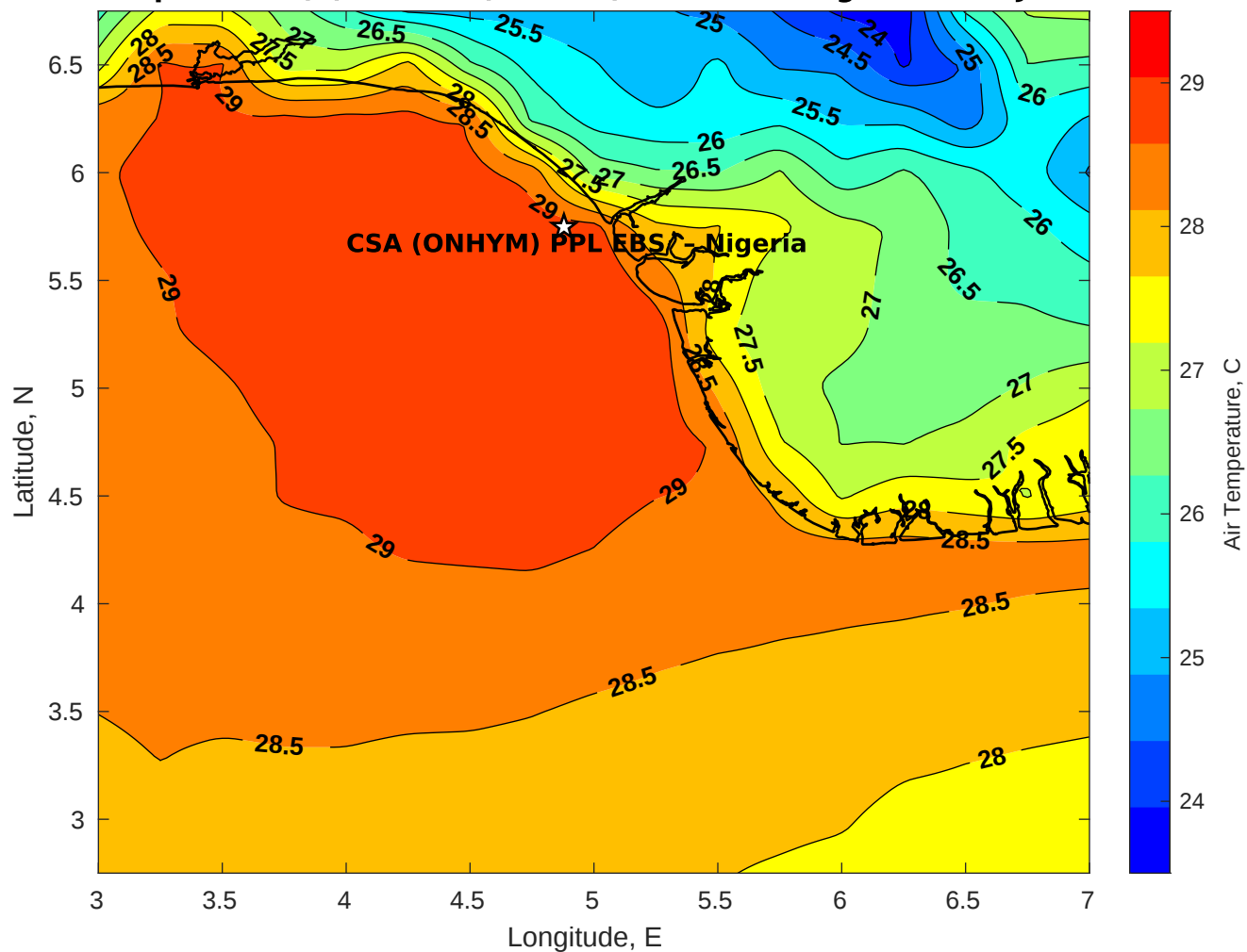
Air Temperature (C) for CSA (ONHYM) PPL EBS - Nigeria at 06-Jan-2026
