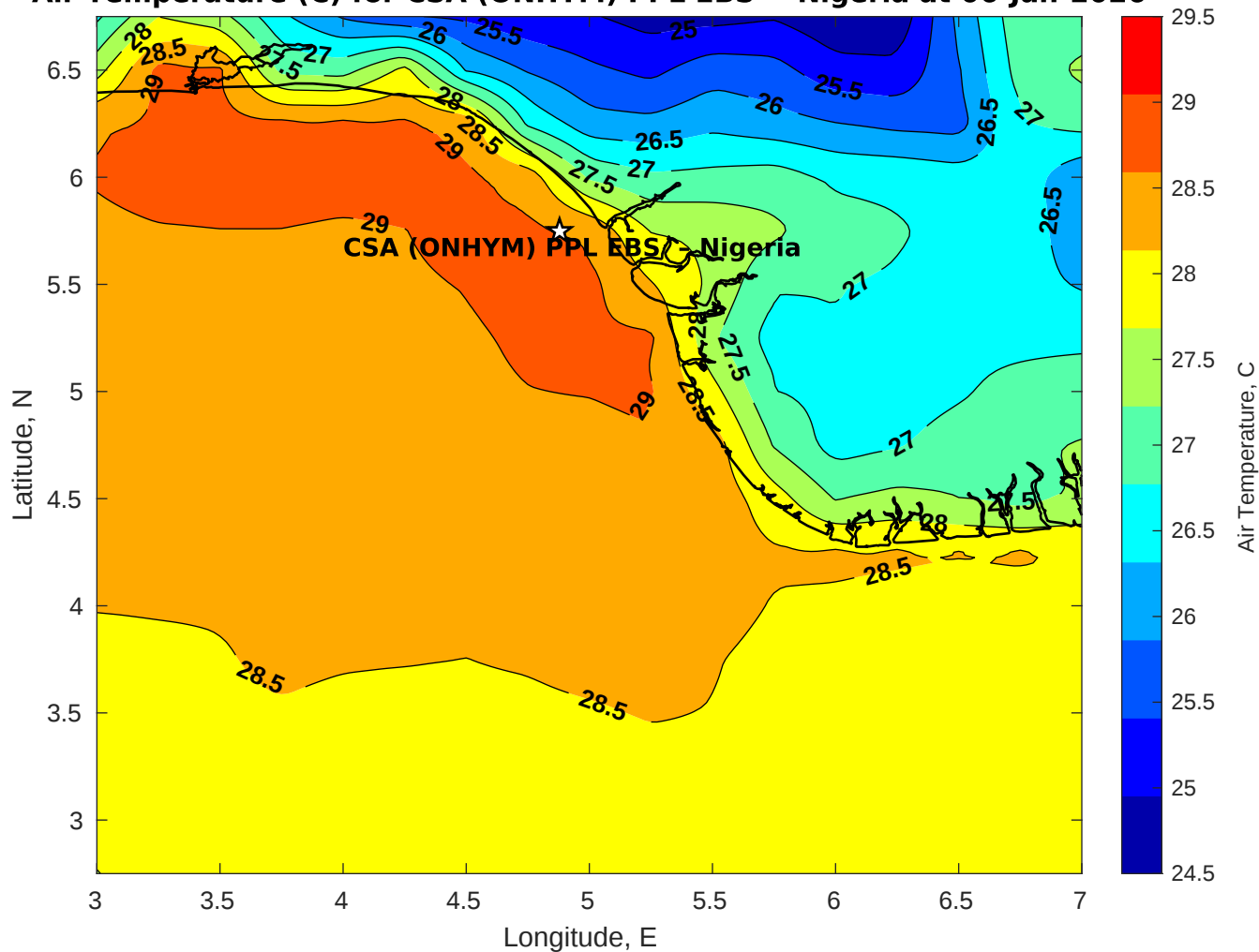
Air Temperature (C) for CSA (ONHYM) PPL EBS - Nigeria at 06-Jan-2026
