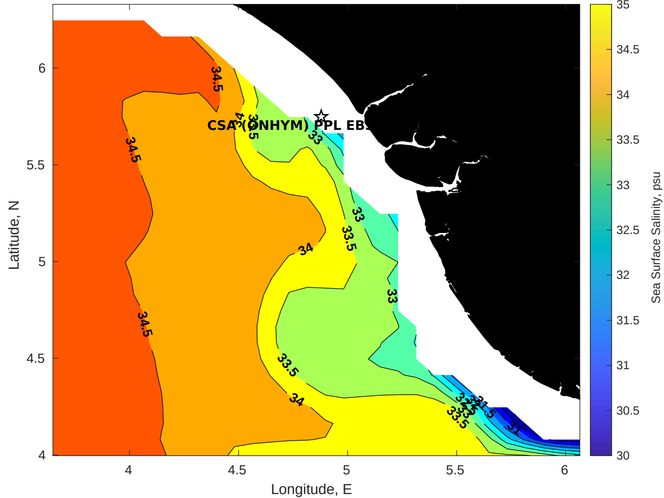
Surface Salinity for CSA (ONHYM) PPL EBS - Nigeria at 05-Jan-2026 00:00:00
