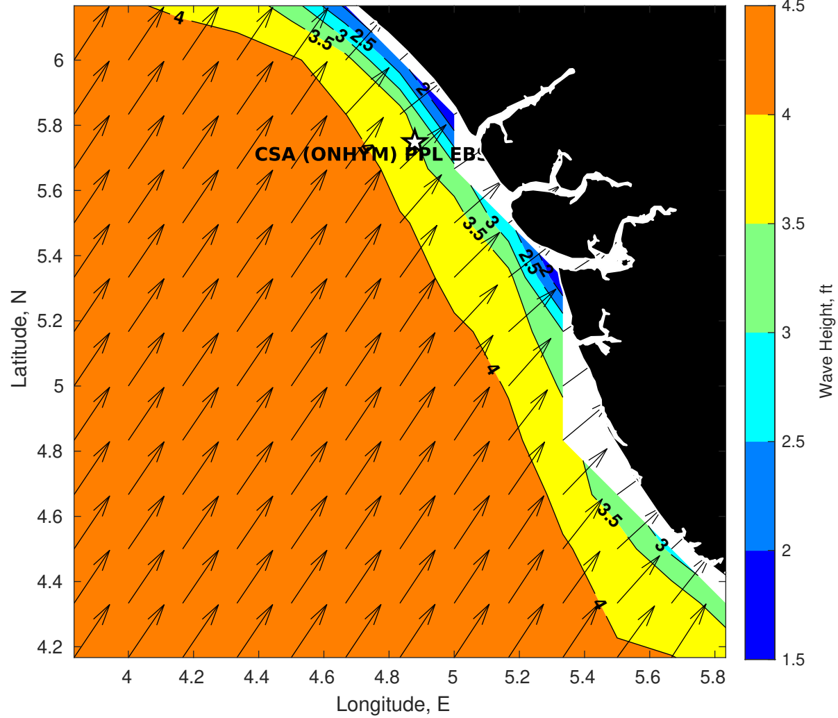
GFS Wave Height (ft) for CSA (ONHYM) PPL EBS - Nigeria at 06-Jan-2026 09:00:00
