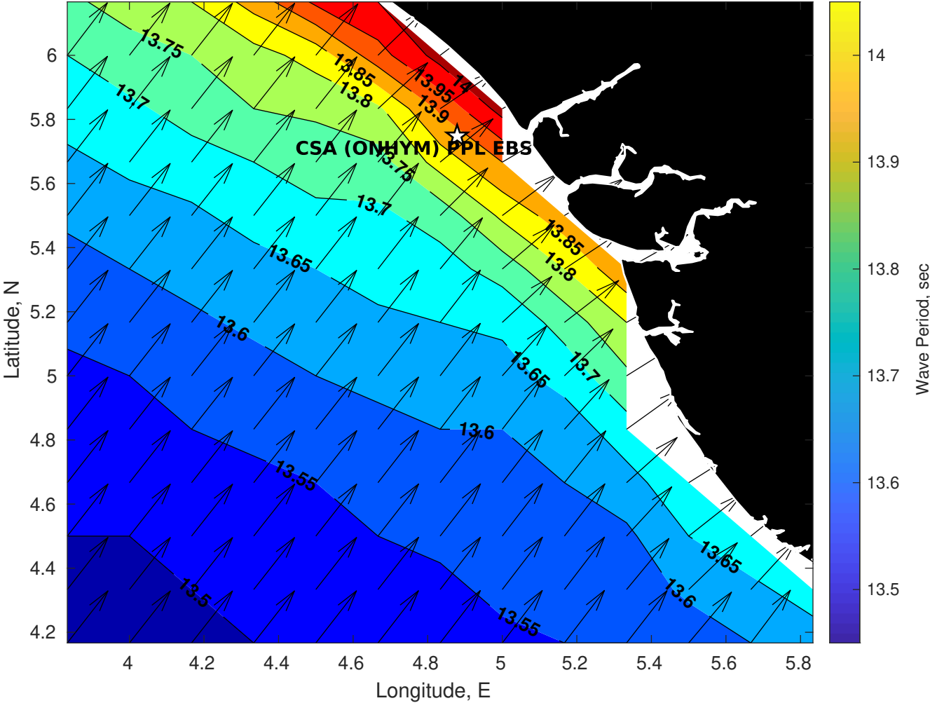
GFS Wave Period (sec) for CSA (ONHYM) PPL EBS - Nigeria at 06-Jan-2026 09:00:00
