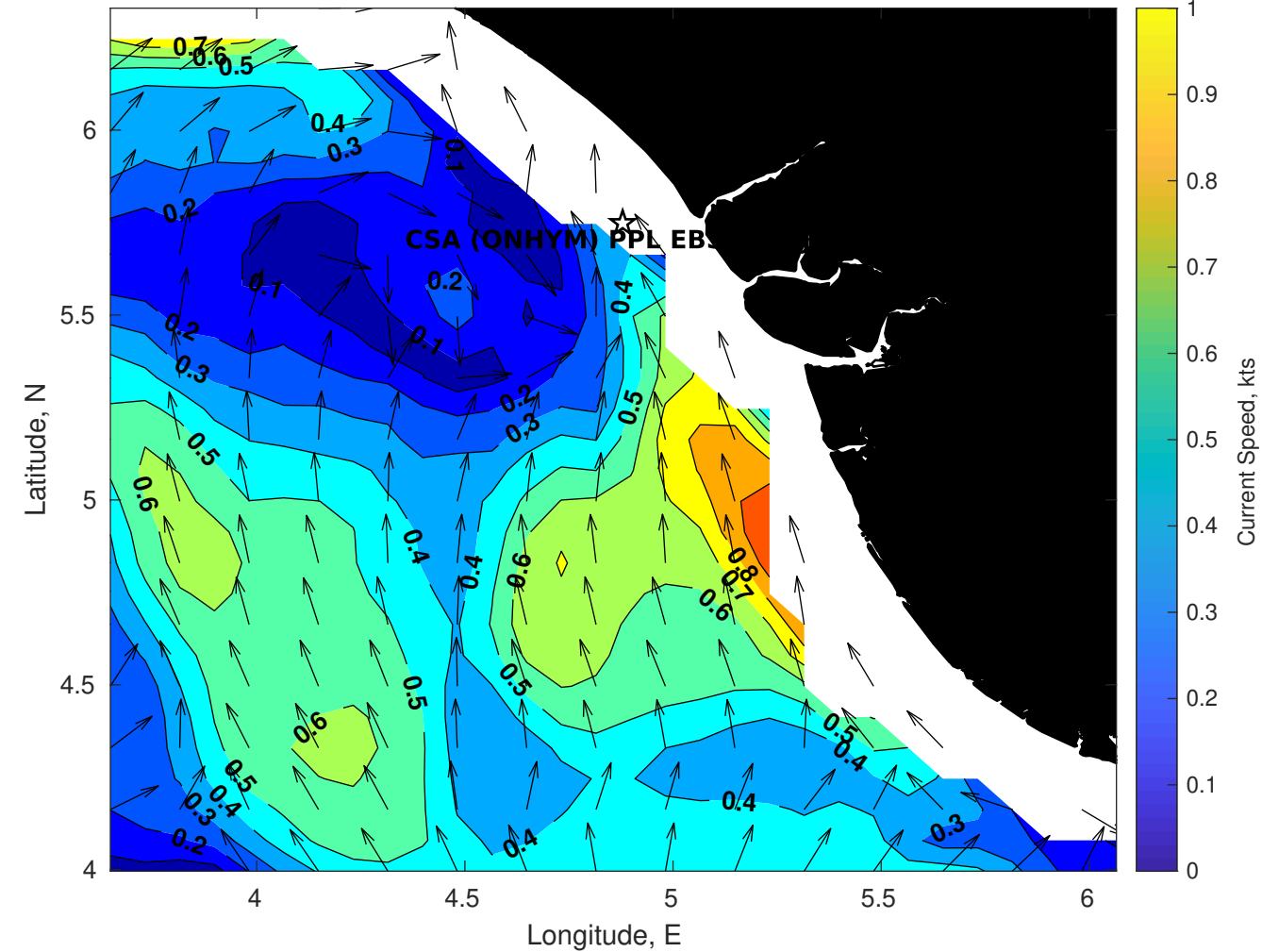
Surface Currents for CSA (ONHYM) PPL EBS - Nigeria at 05-Jan-2026 00:00:00
