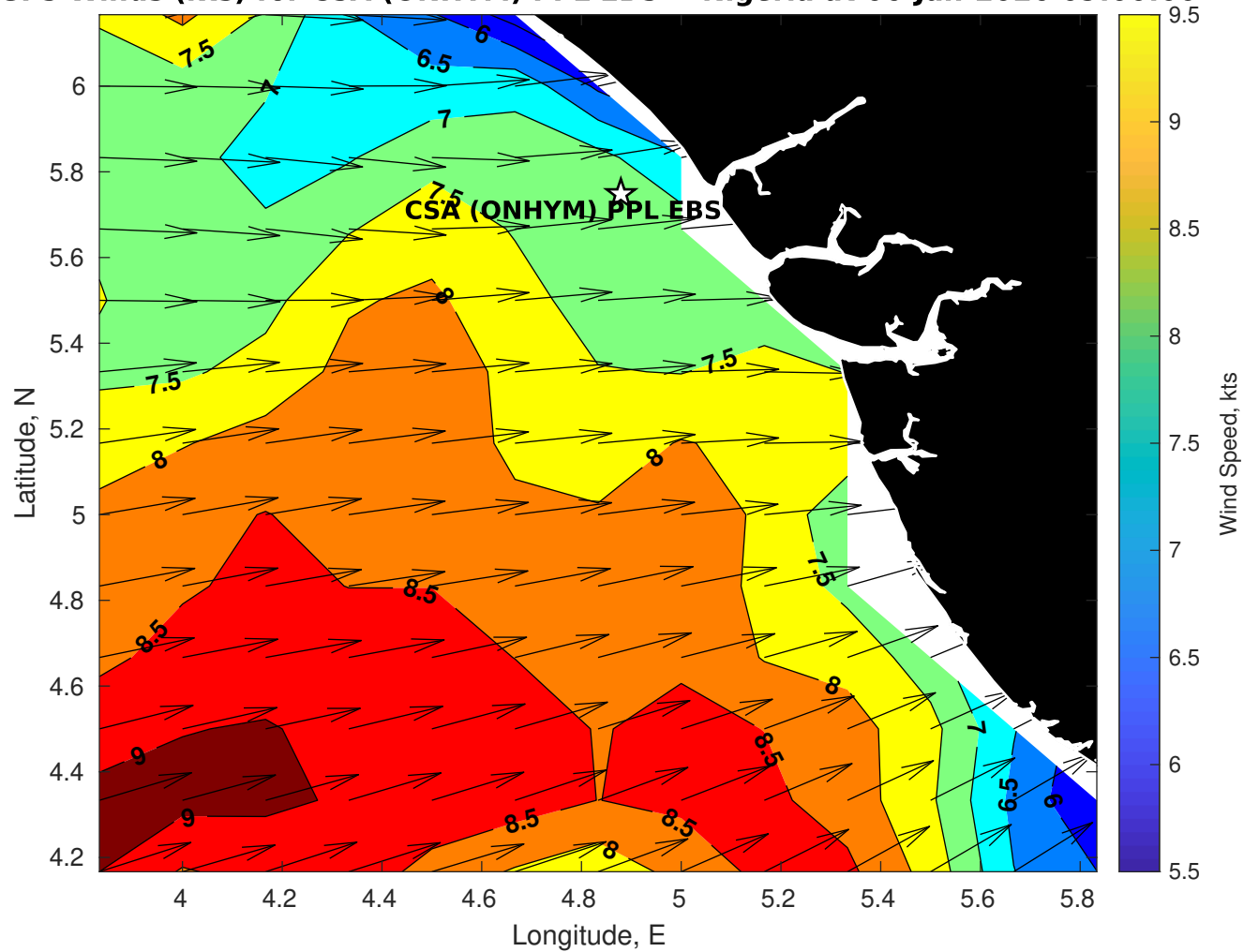
GFS Winds (kts) for CSA (ONHYM) PPL EBS - Nigeria at 06-Jan-2026 09:00:00
