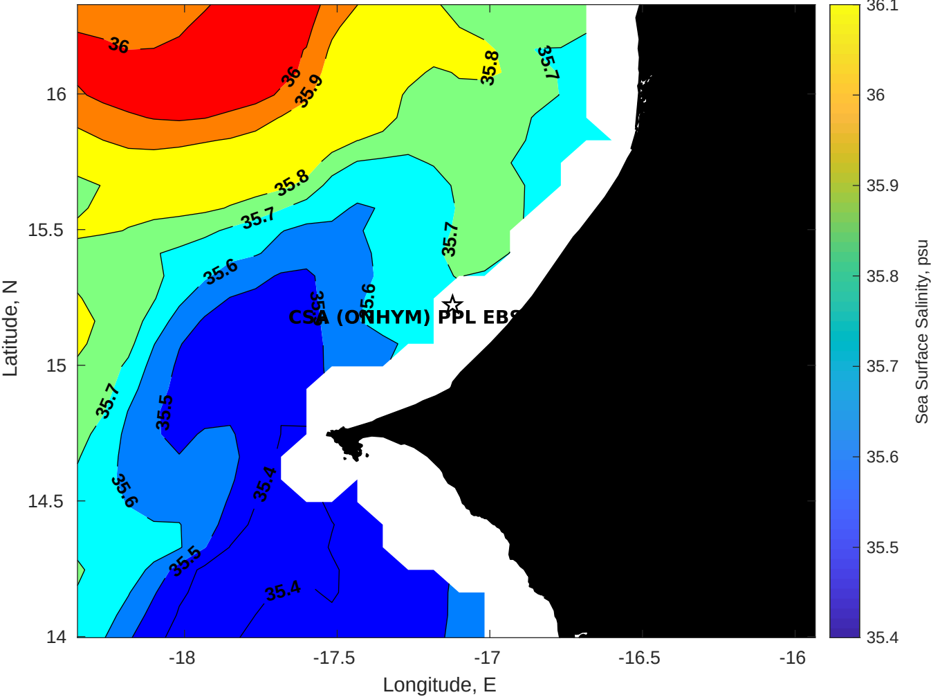
Surface Salinity for CSA (ONHYM) PPL EBS - Senegal at 05-Jan-2026 00:00:00
