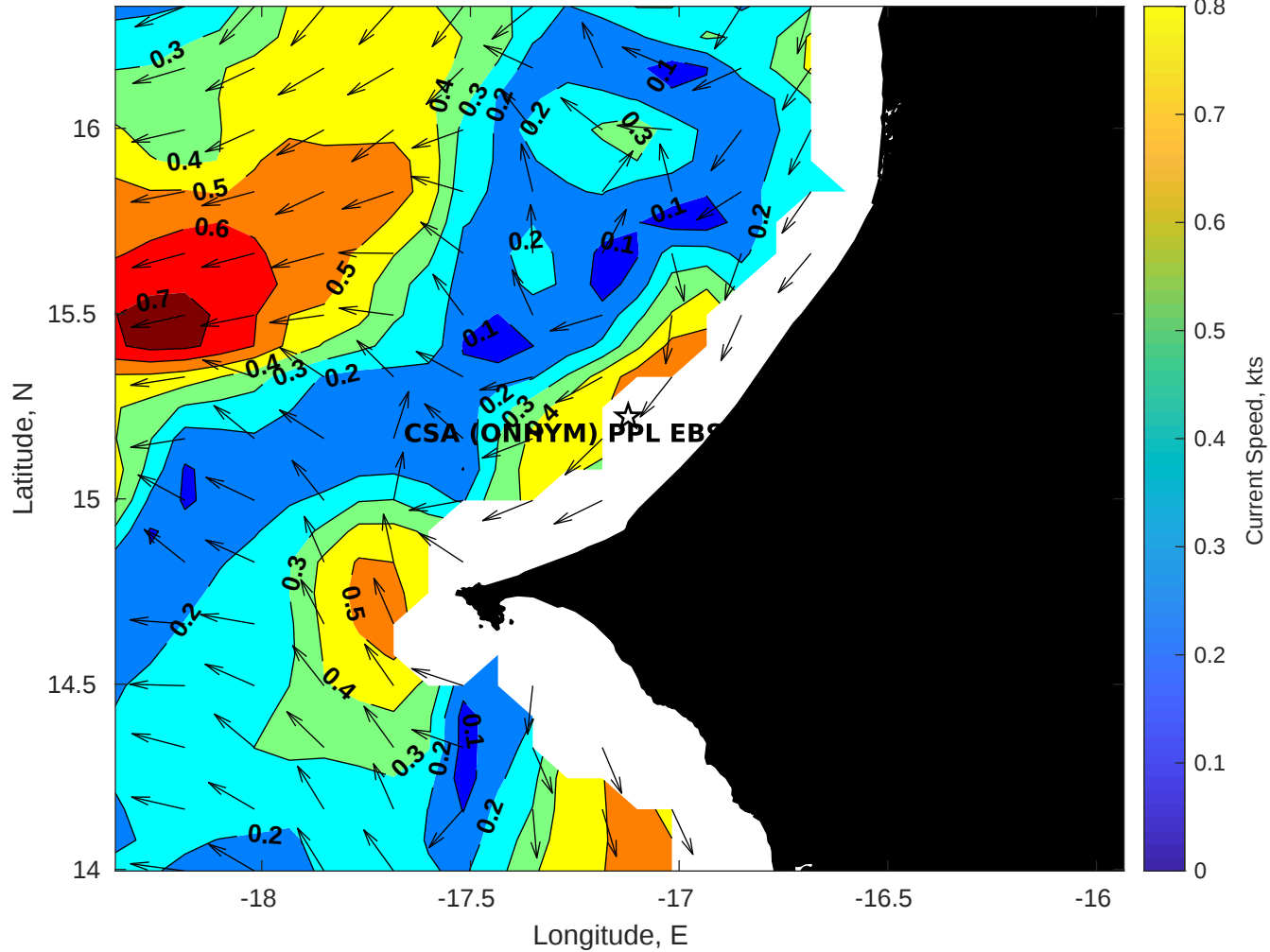
Surface Currents for CSA (ONHYM) PPL EBS - Senegal at 05-Jan-2026 00:00:00
