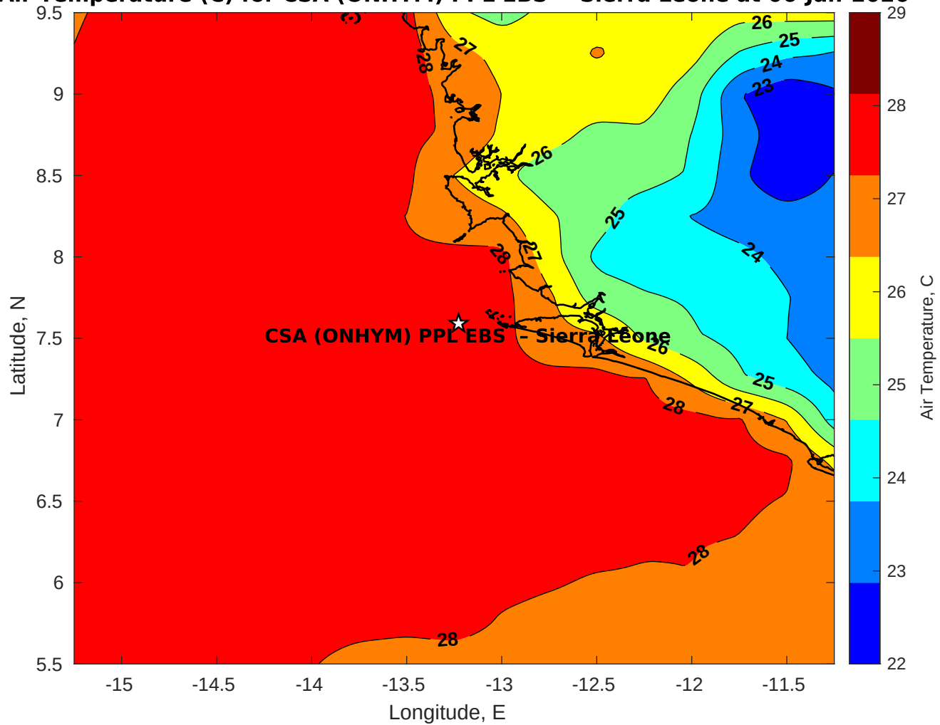
Air Temperature (C) for CSA (ONHYM) PPL EBS - Sierra Leone at 06-Jan-2026
