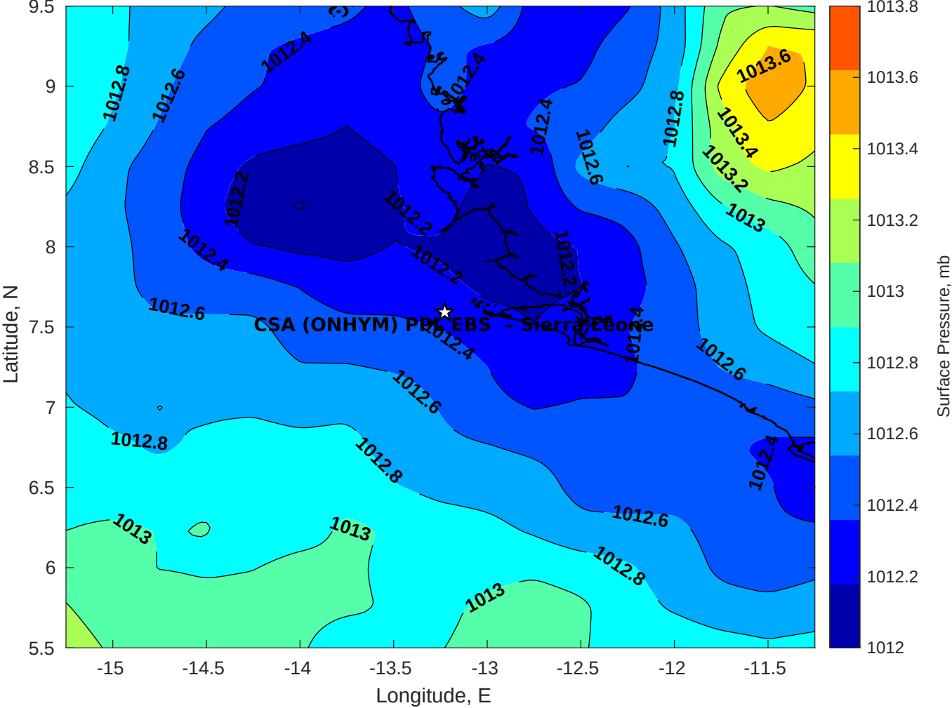
Surface Pressure (mb) for CSA (ONHYM) PPL EBS - Sierra Leone at 07-Jan-2026 00:00:00
