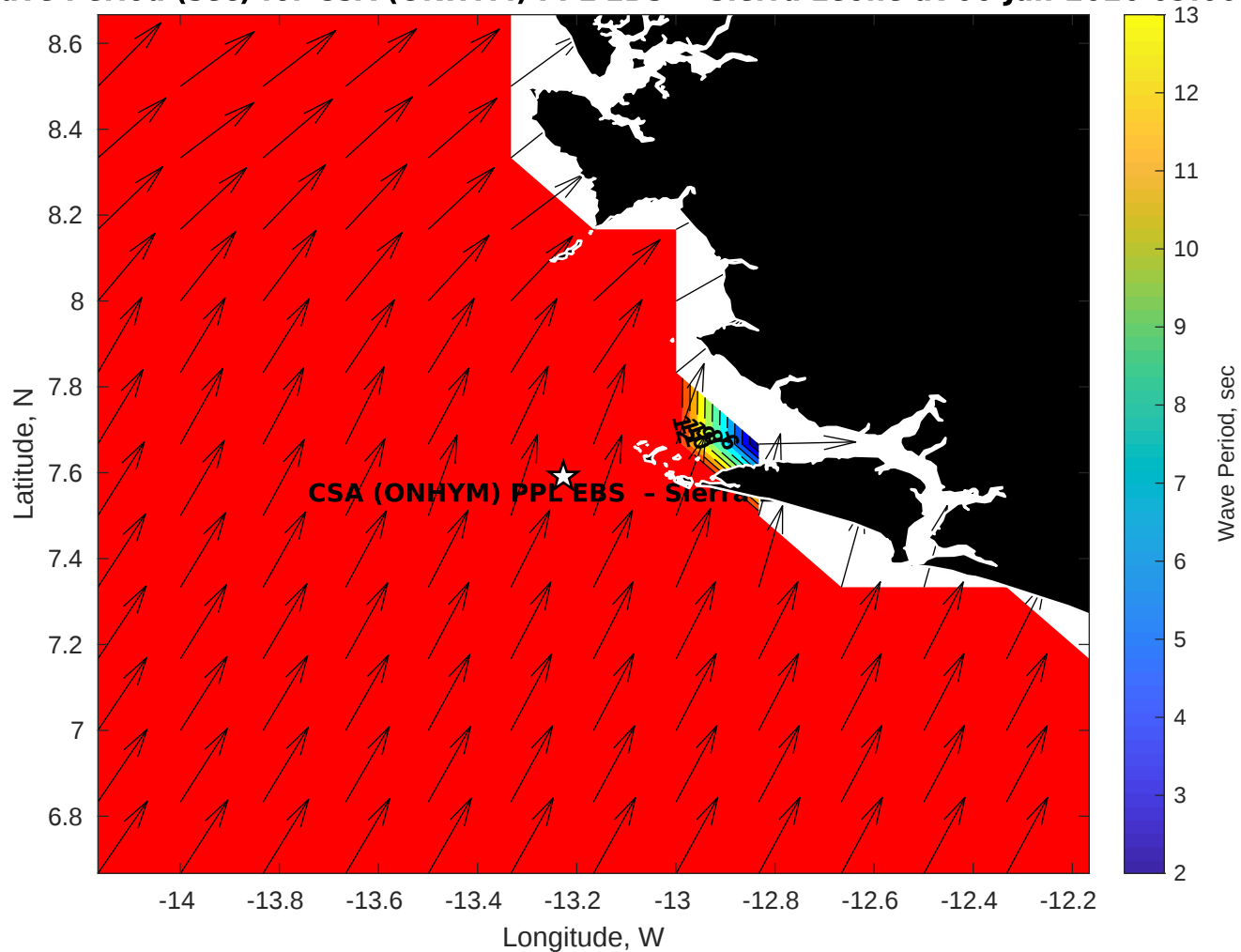
GFS Wave Period (sec) for CSA (ONHYM) PPL EBS - Sierra Leone at 06-Jan-2026 09:00:00
