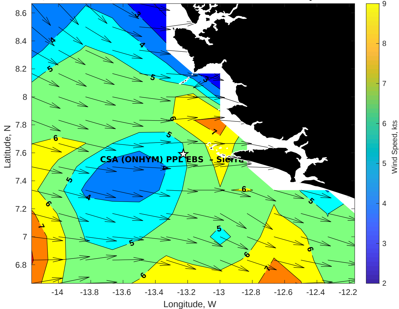
GFS Winds (kts) for CSA (ONHYM) PPL EBS - Sierra Leone at 06-Jan-2026 09:00:00
