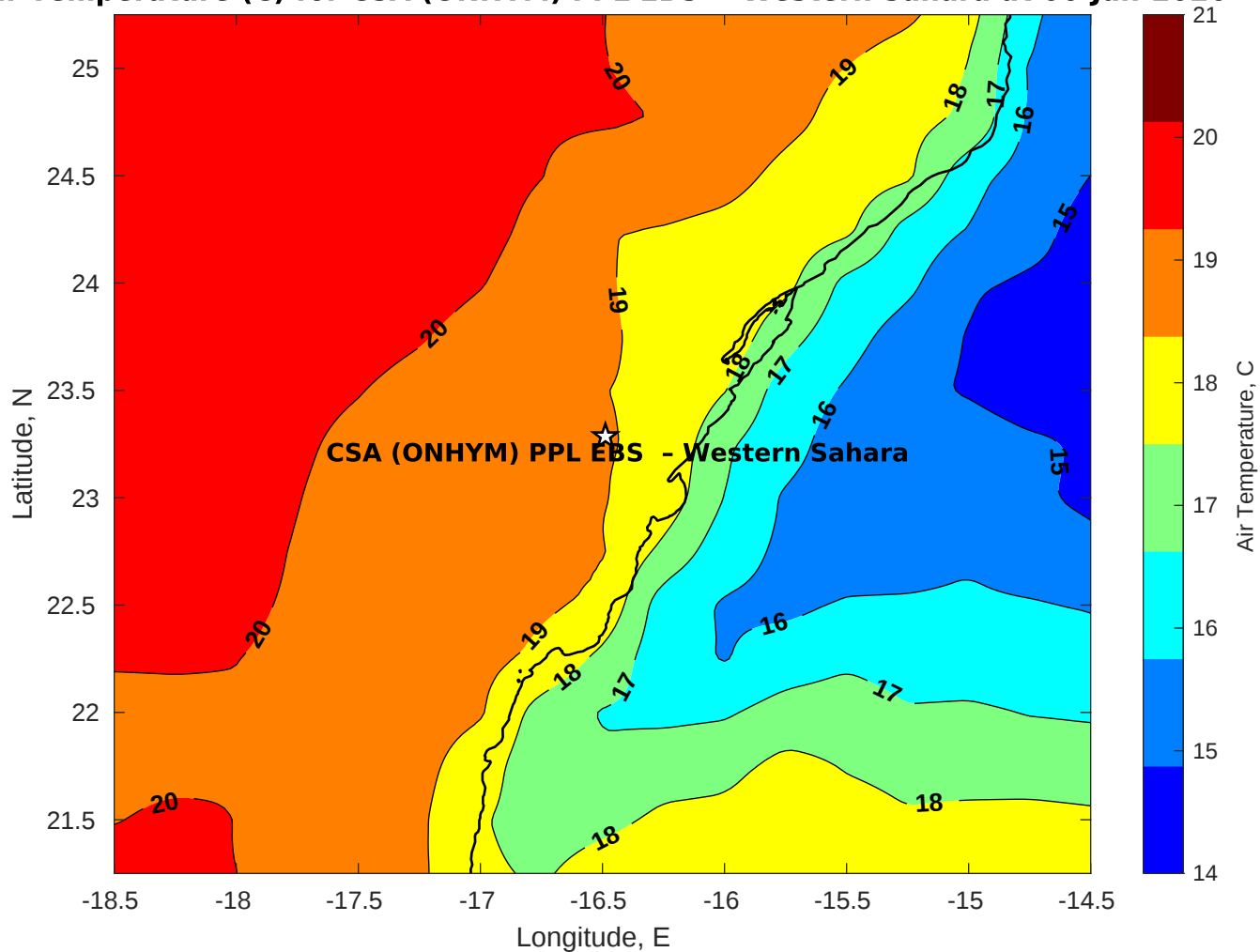
Air Temperature (C) for CSA (ONHYM) PPL EBS - Western Sahara at 06-Jan-2026
