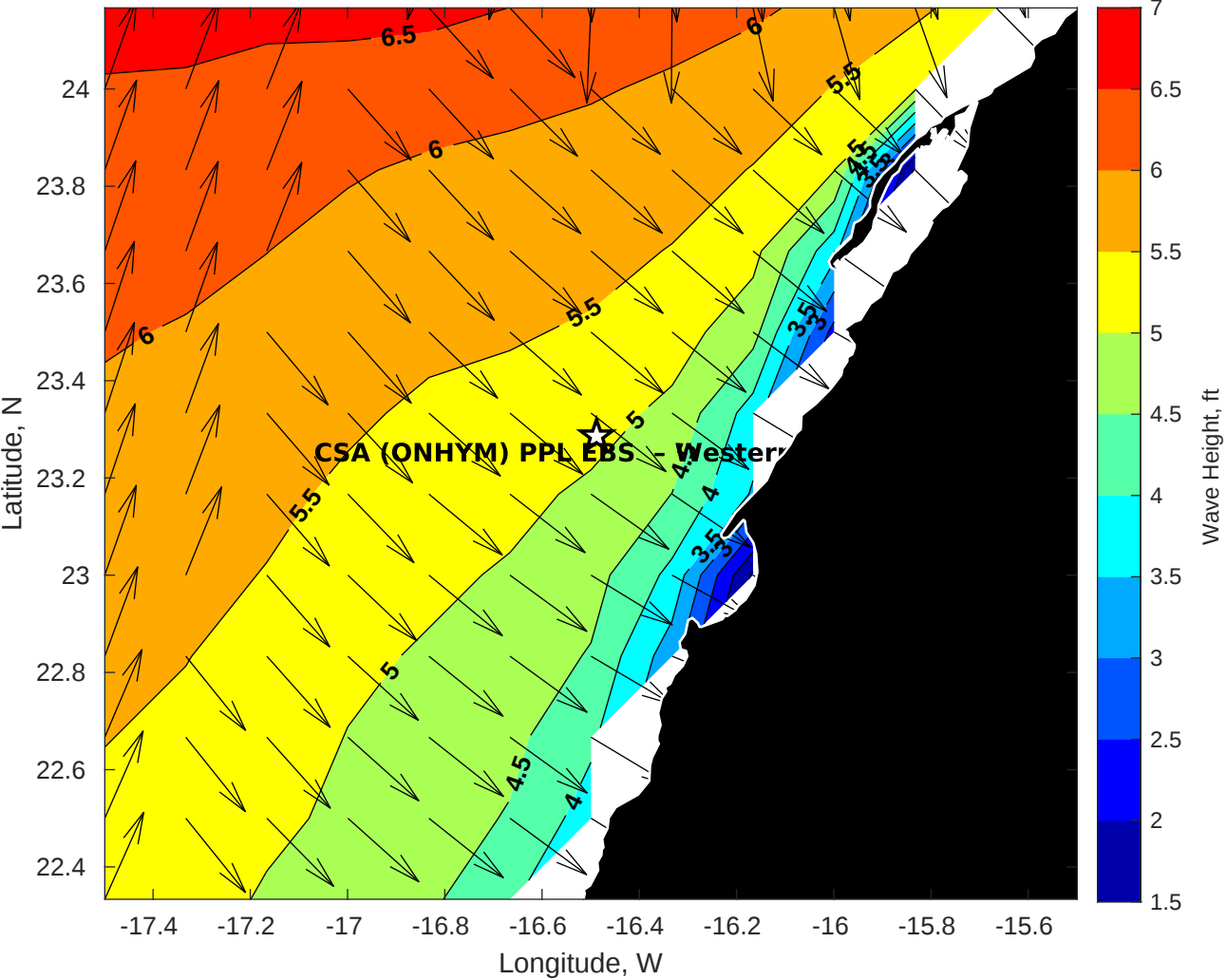
GFS Wave Height (ft) for CSA (ONHYM) PPL EBS - Western Sahara at 06-Jan-2026 09:00:00
