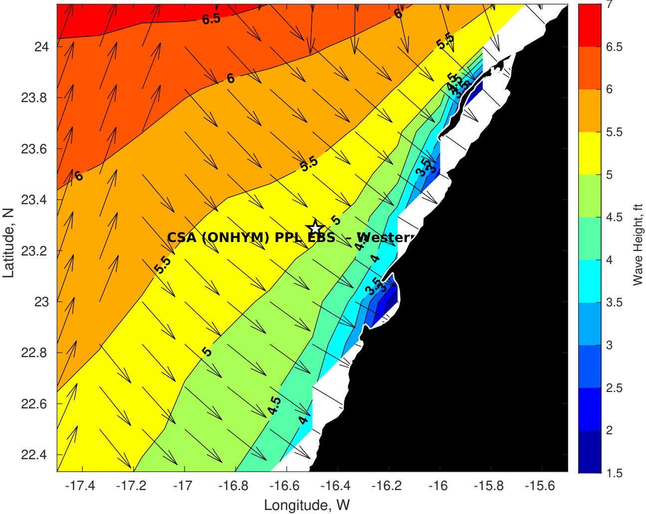
GFS Wave Height (ft) for CSA (ONHYM) PPL EBS - Western Sahara at 06-Jan-2026 09:00:00
