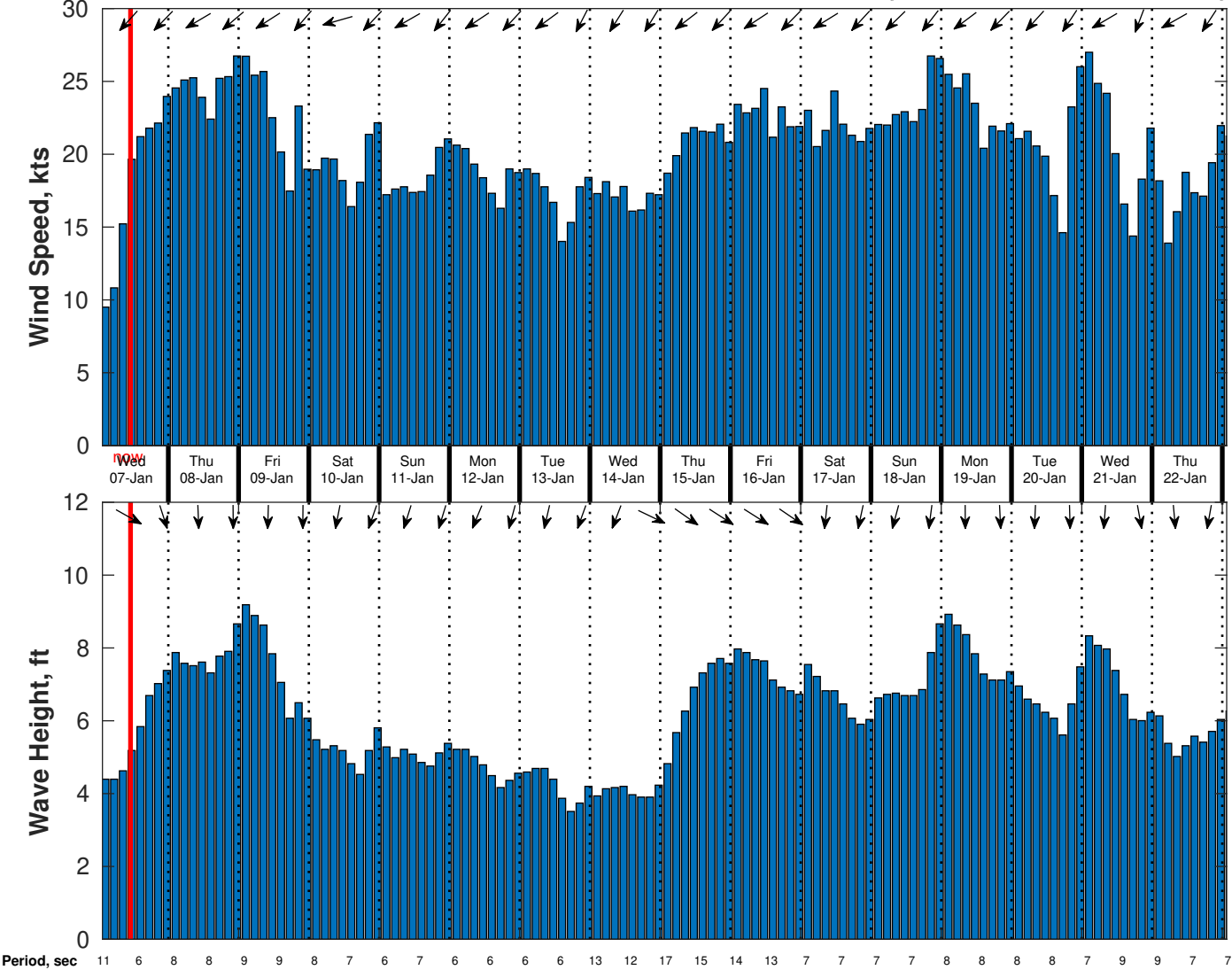
Wind & Wave Forecast for CSA (ONHYM) PPL EBS - Western Sahara from 06-Jan-2026 01:00:00 to 22-Jan-2026 01:00:00
