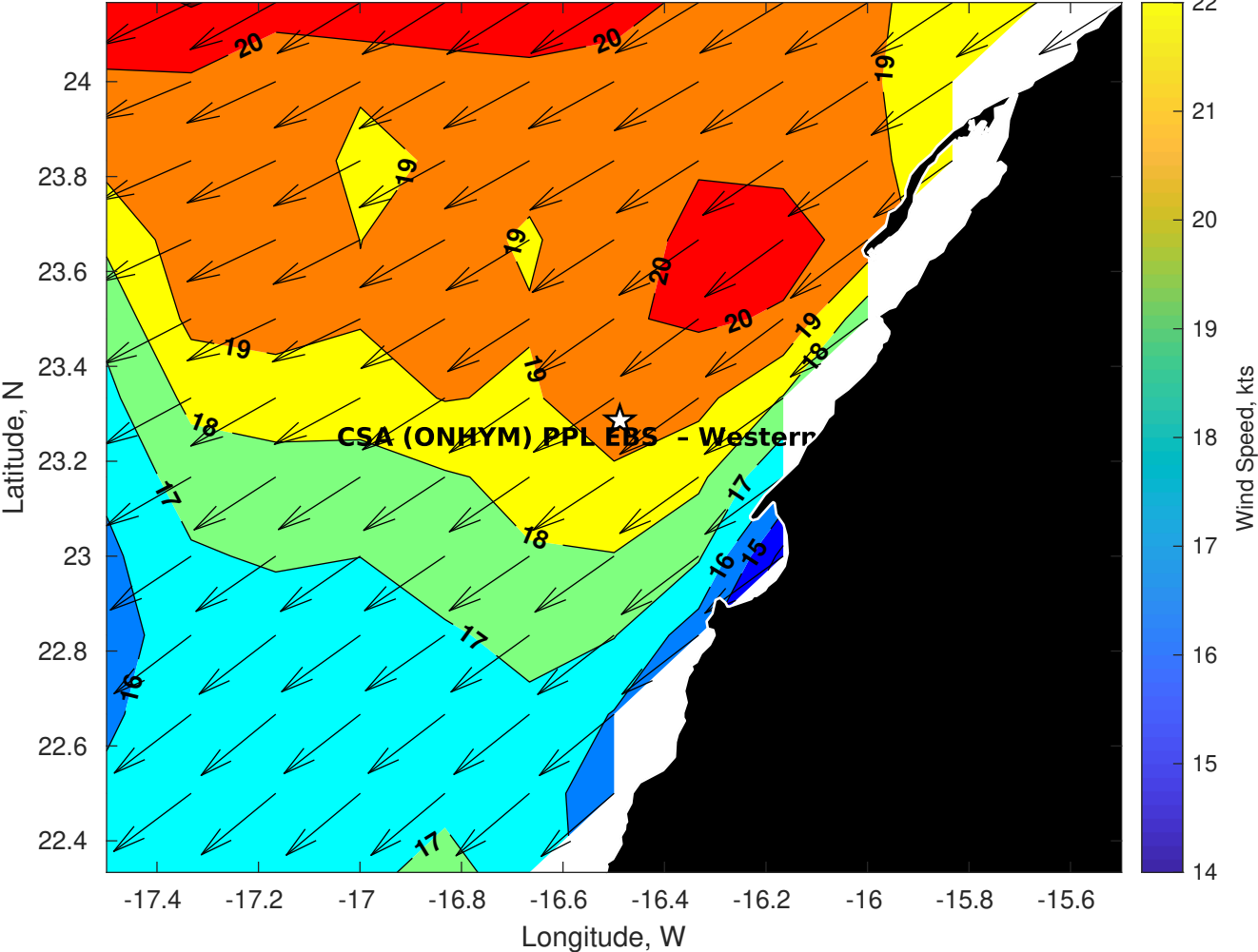
GFS Winds (kts) for CSA (ONHYM) PPL EBS - Western Sahara at 06-Jan-2026 09:00:00
