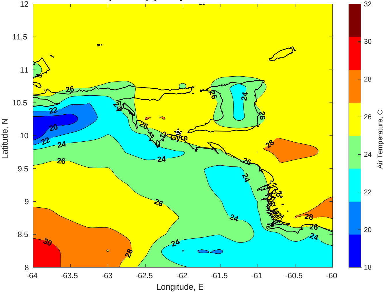
Air Temperature (C) for Gyre at 06-Jan-2026
