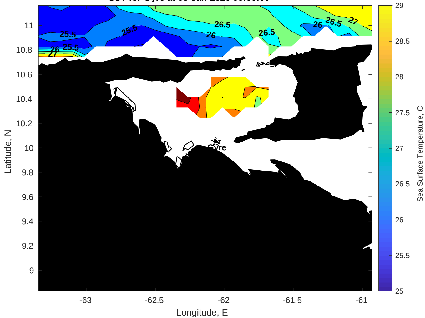
SST for Gyre at 05-Jan-2026 00:00:00
