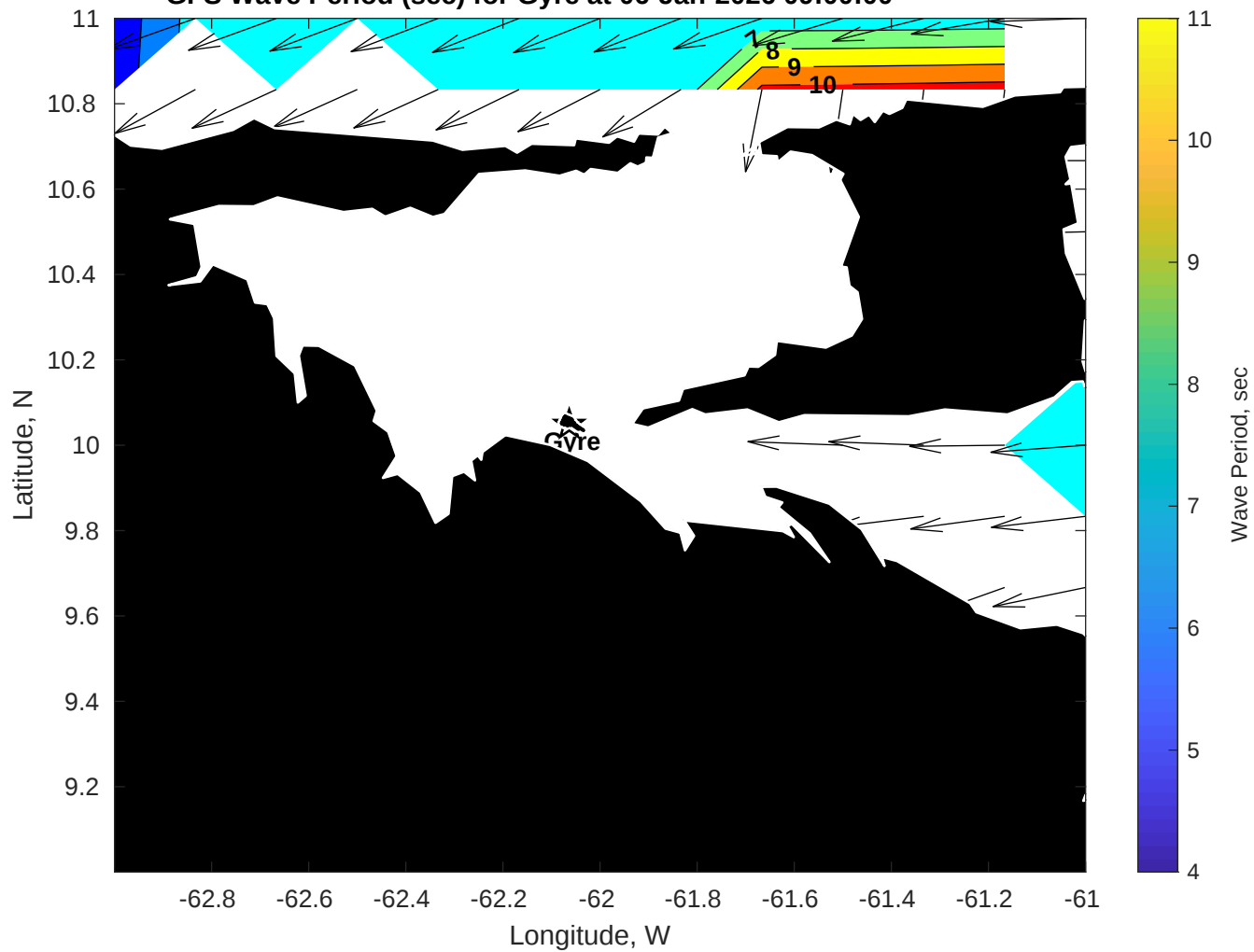
GFS Wave Period (sec) for Gyre at 06-Jan-2026 09:00:00
