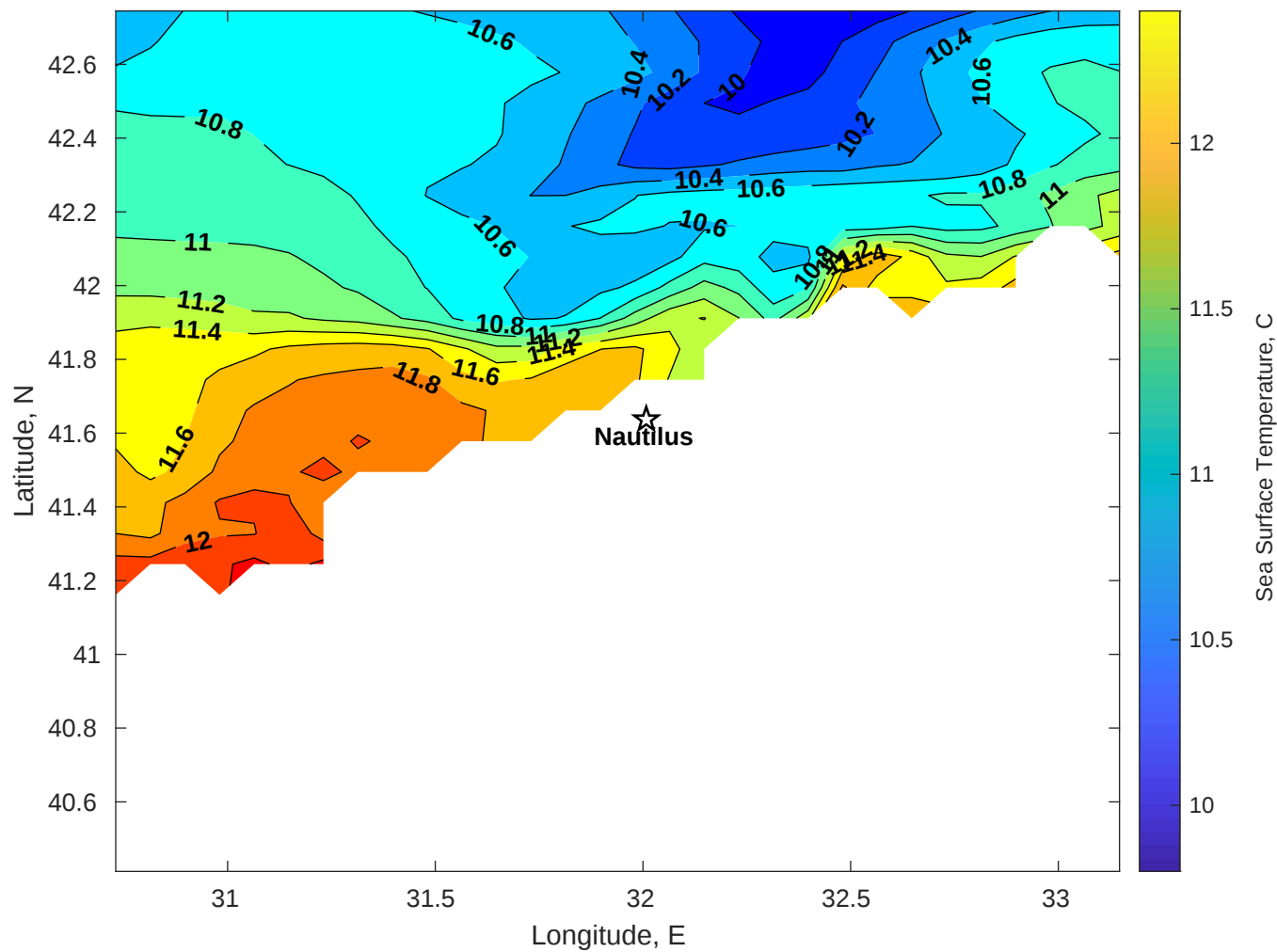
SST for Nautilus at 05-Jan-2026 00:00:00
