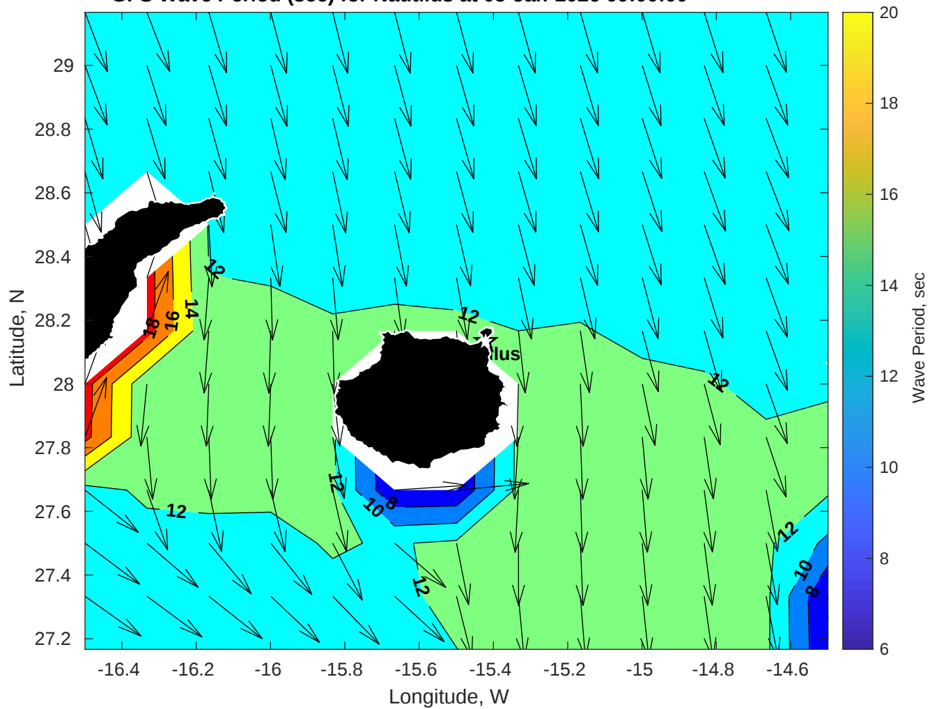
GFS Wave Period (sec) for Nautilus at 05-Jan-2026 09:00:00
