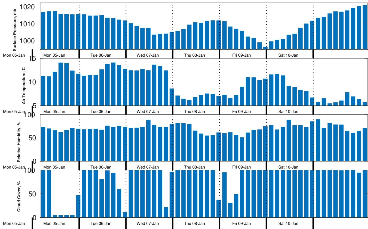
Met Forecast for Nautilus from 06-Jan-2026 00:00:00 to 13-Jan-2026 00:00:00
