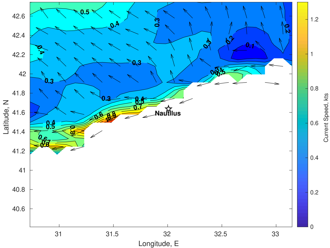
Surface Currents for Nautilus at 05-Jan-2026 00:00:00
