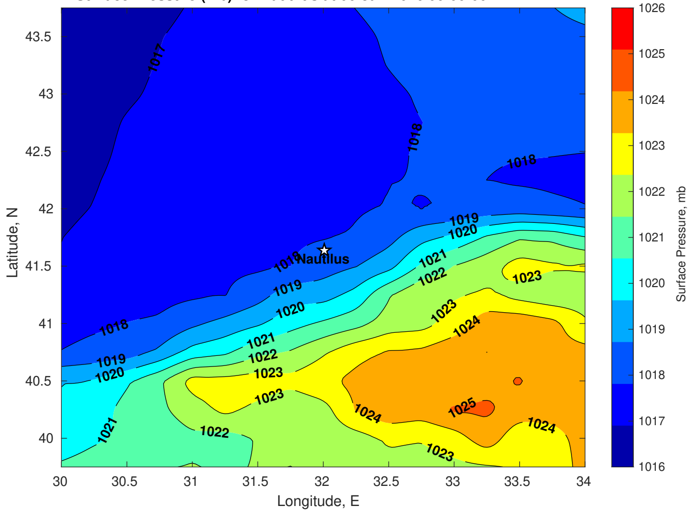
Surface Pressure (mb) for Nautilus at 06-Jan-2026 00:00:00
