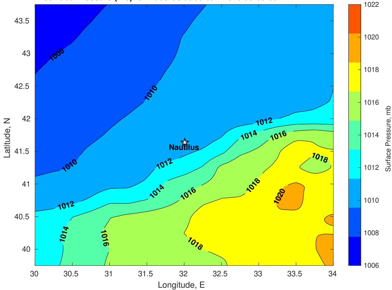
Surface Pressure (mb) for Nautilus at 08-Jan-2026 00:00:00
