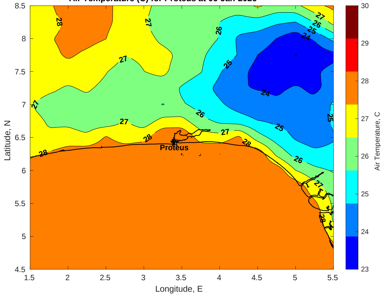
Air Temperature (C) for Proteus at 06-Jan-2026
