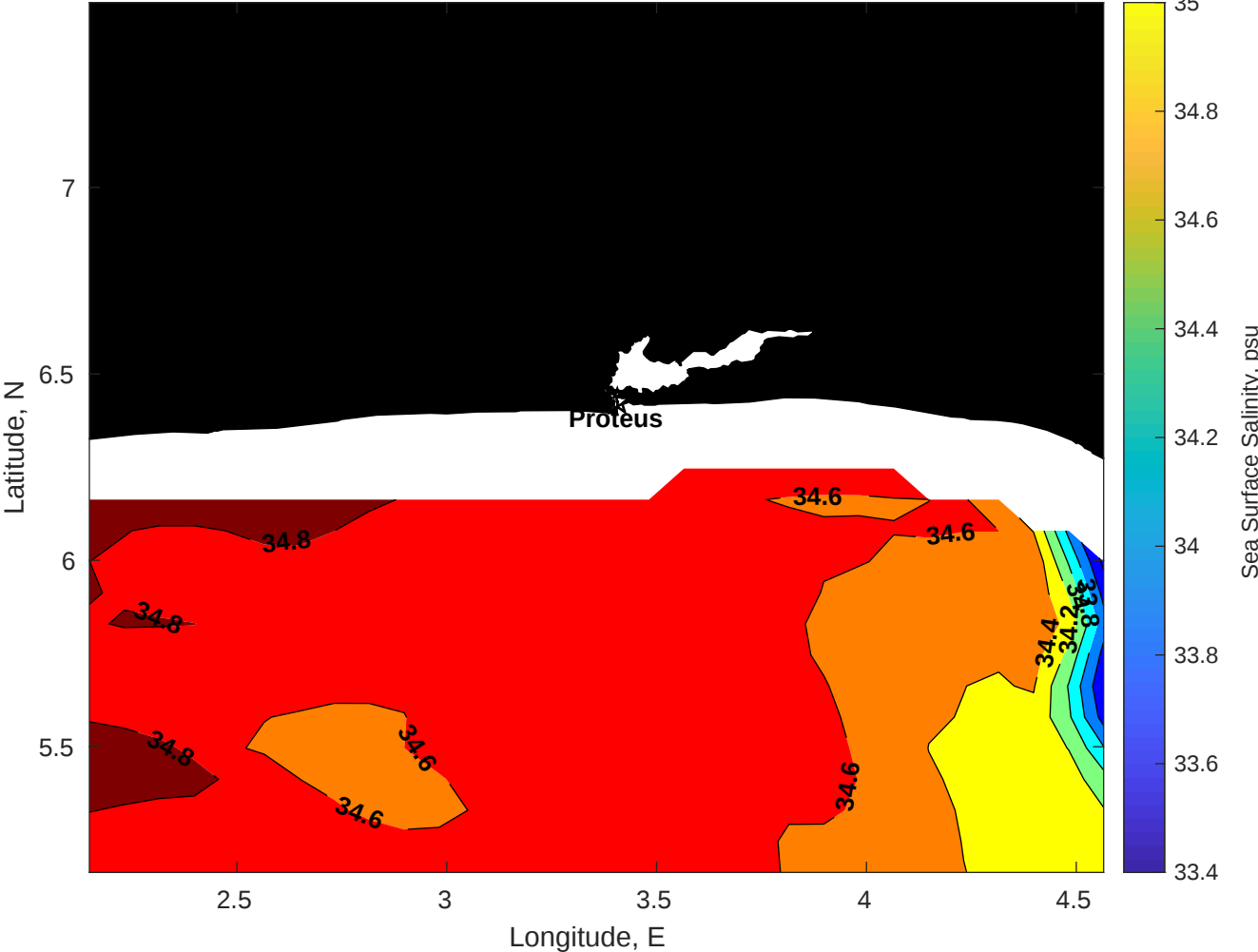
Surface Salinity for Proteus at 05-Jan-2026 00:00:00
