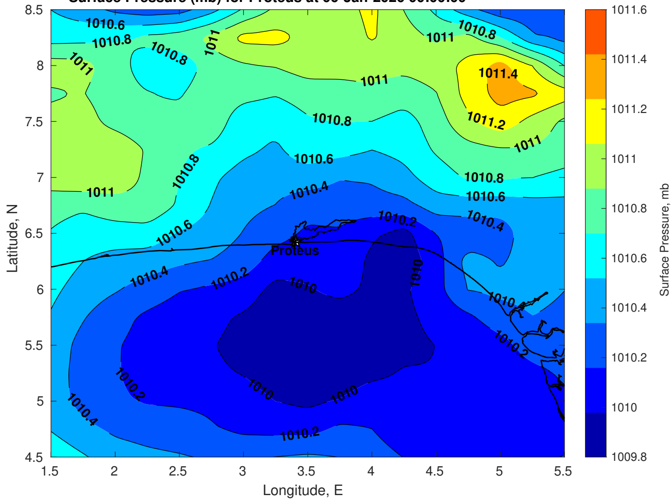
Surface Pressure (mb) for Proteus at 06-Jan-2026 00:00:00
