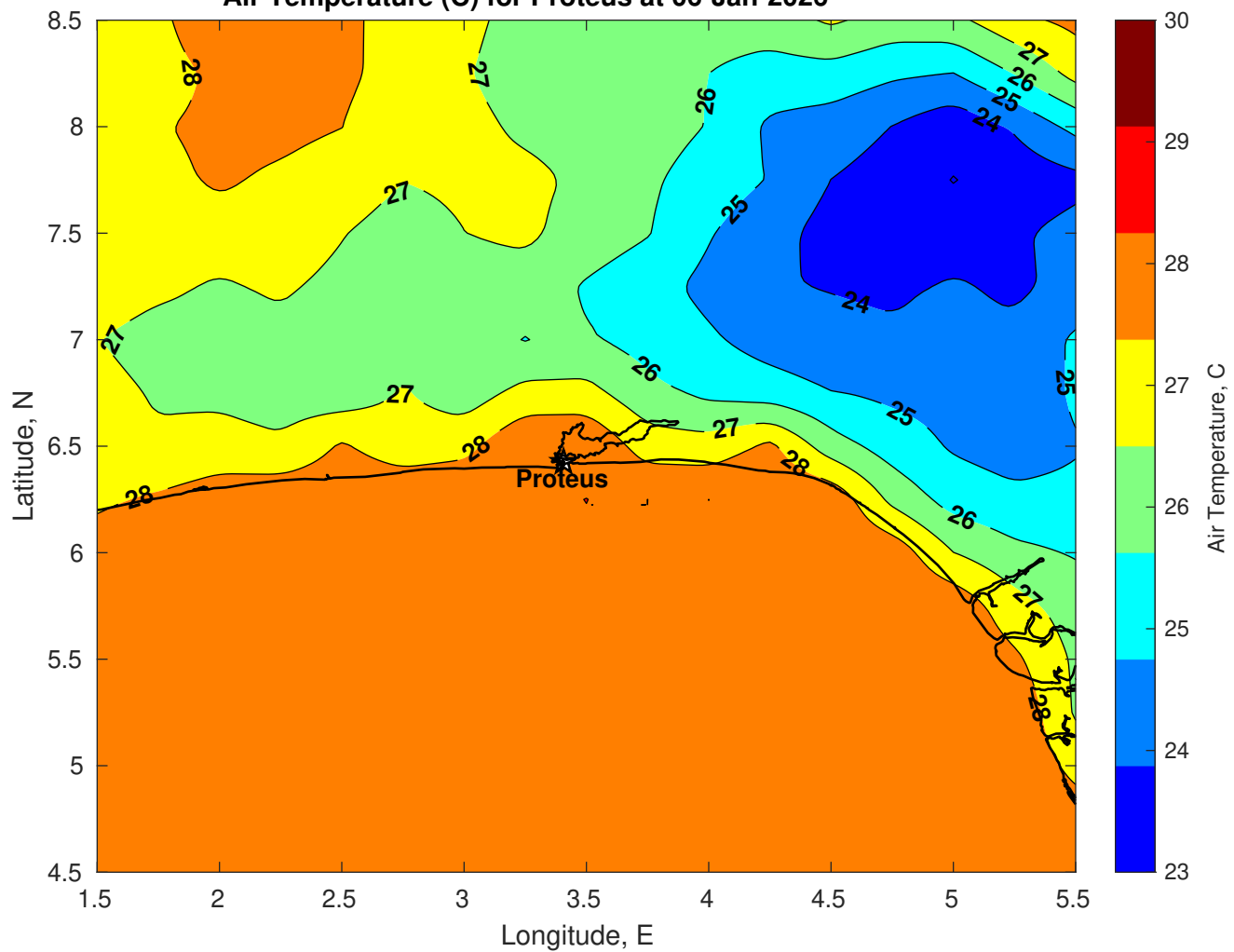
Air Temperature (C) for Proteus at 06-Jan-2026
