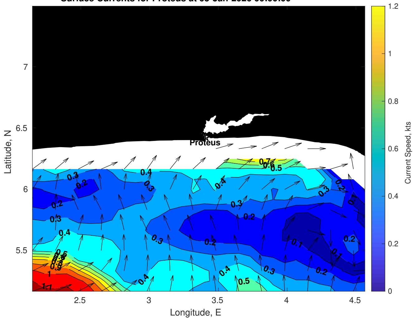
Surface Currents for Proteus at 05-Jan-2026 00:00:00
