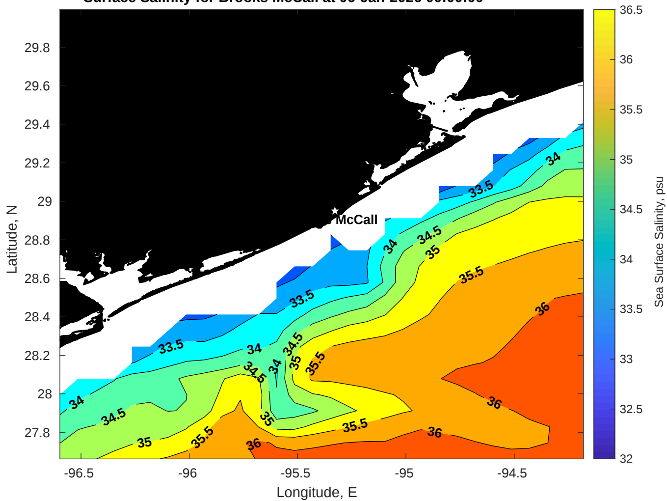
Surface Salinity for Brooks McCall at 06-Jan-2026 00:00:00
