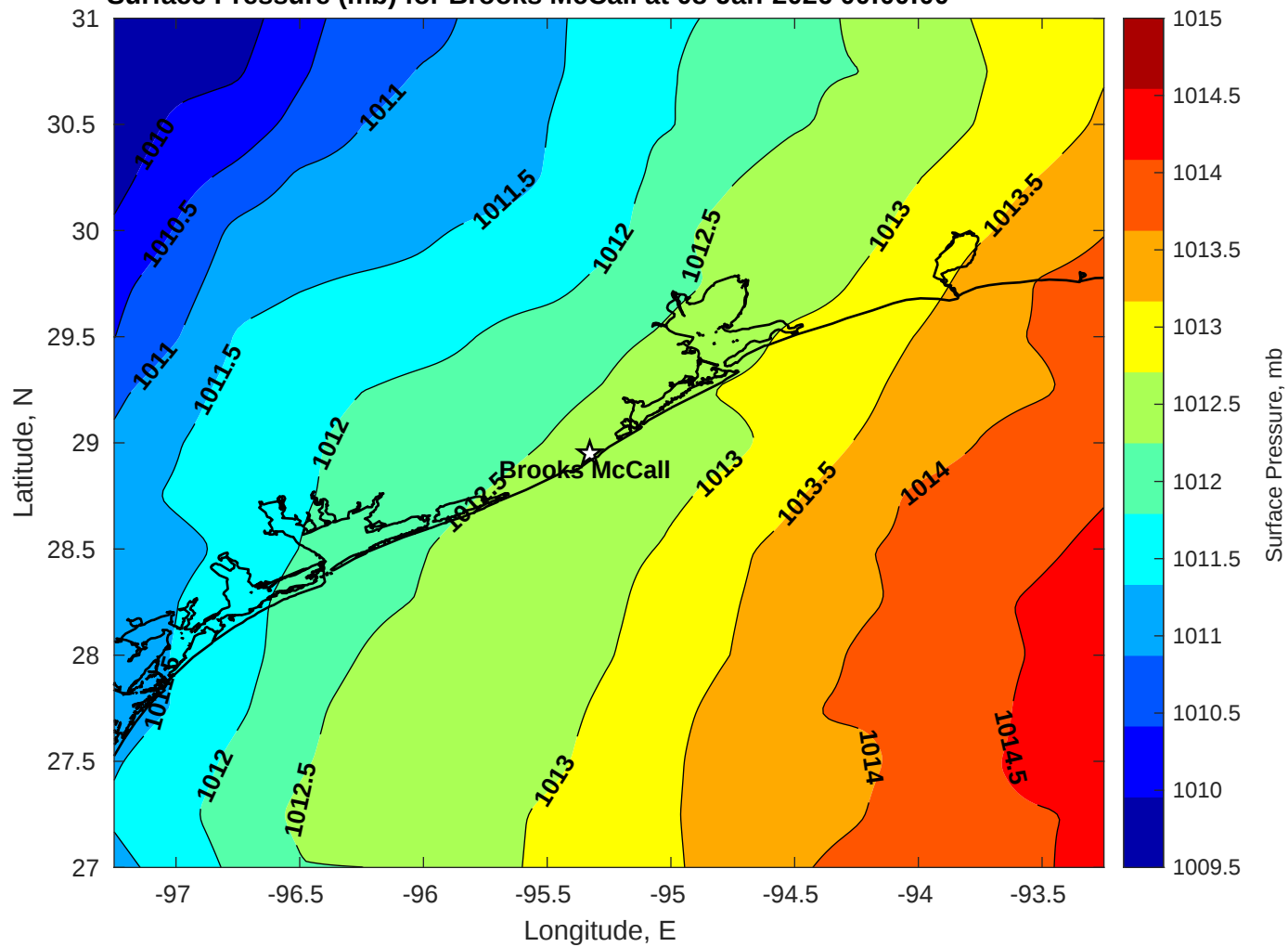
Surface Pressure (mb) for Brooks McCall at 08-Jan-2026 00:00:00
