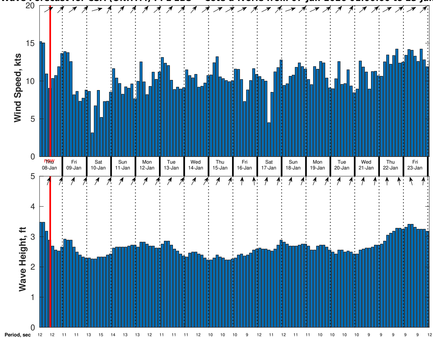
Wind & Wave Forecast for CSA (ONHYM) PPL EBS - Cote d'Ivoire from 07-Jan-2026 01:00:00 to 23-Jan-2026 01:00:00
