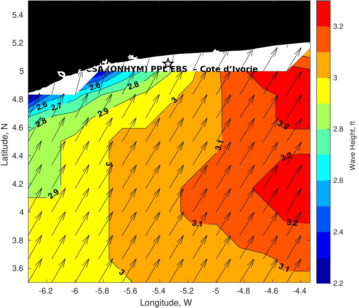
GFS Wave Height (ft) for CSA (ONHYM) PPL EBS - Cote d'Ivoire at 07-Jan-2026 09:00:00
