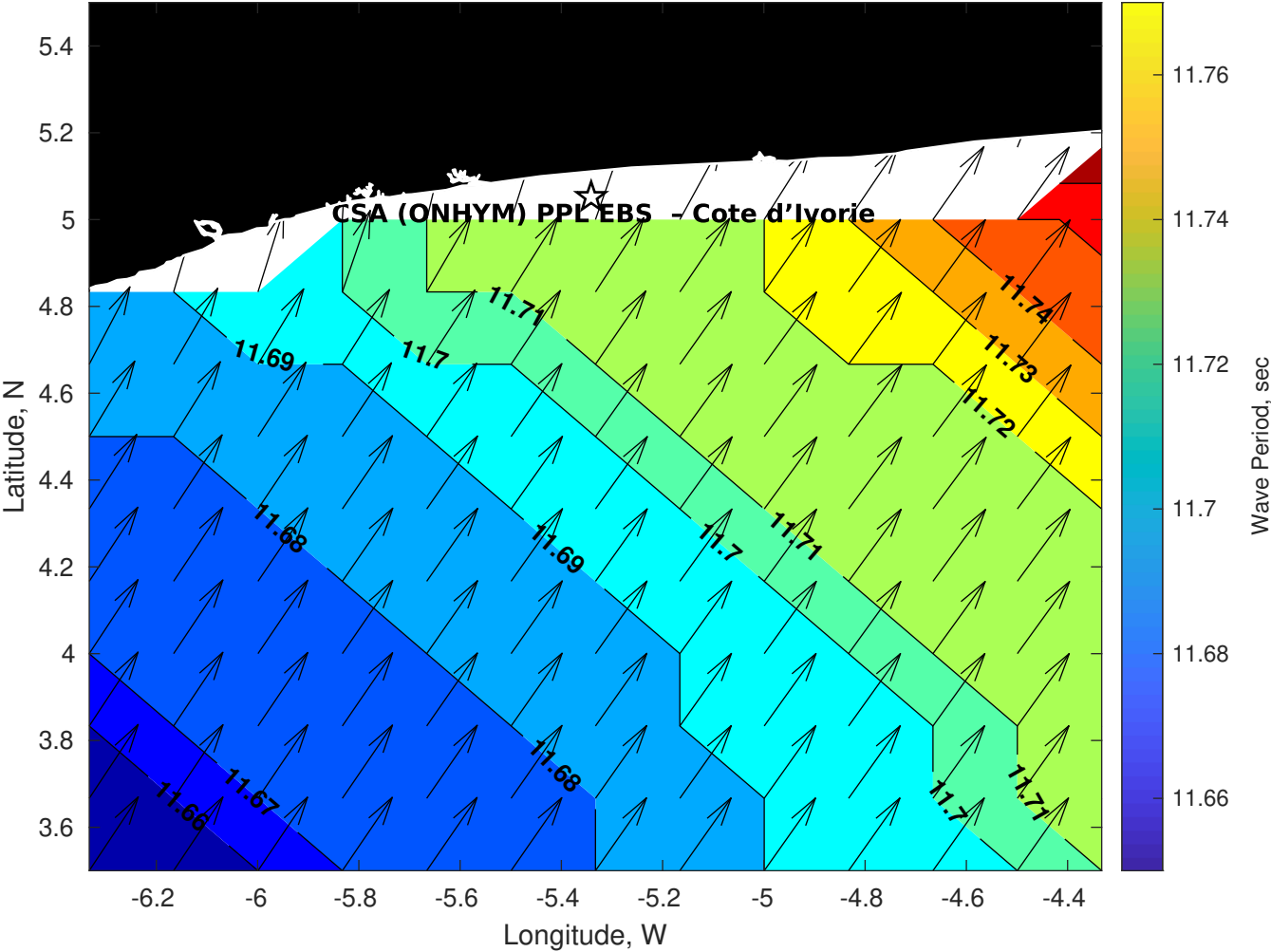
GFS Wave Period (sec) for CSA (ONHYM) PPL EBS - Cote d'Ivoire at 07-Jan-2026 09:00:00
