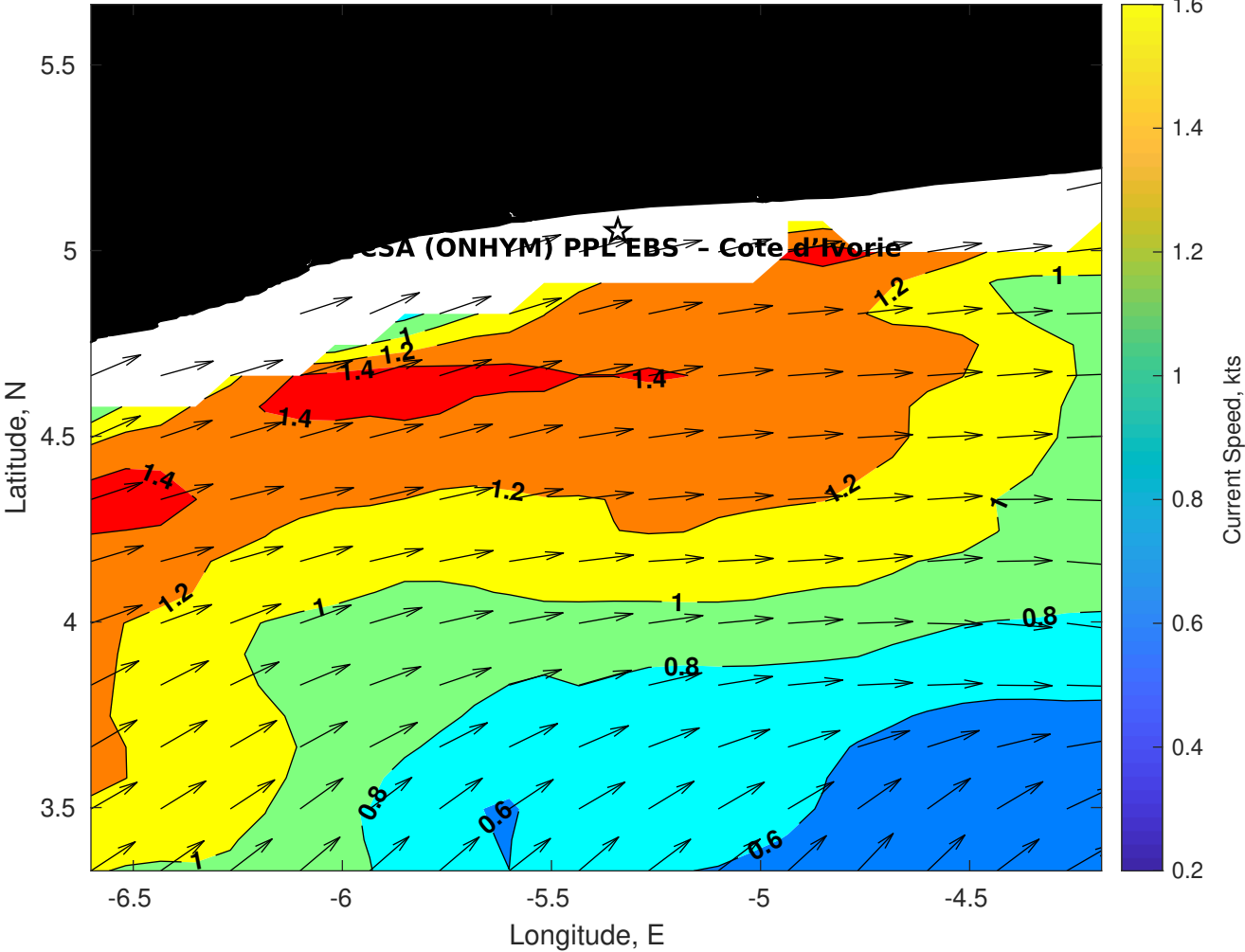
Surface Currents for CSA (ONHYM) PPL EBS - Cote d'Ivoire at 06-Jan-2026 00:00:00
