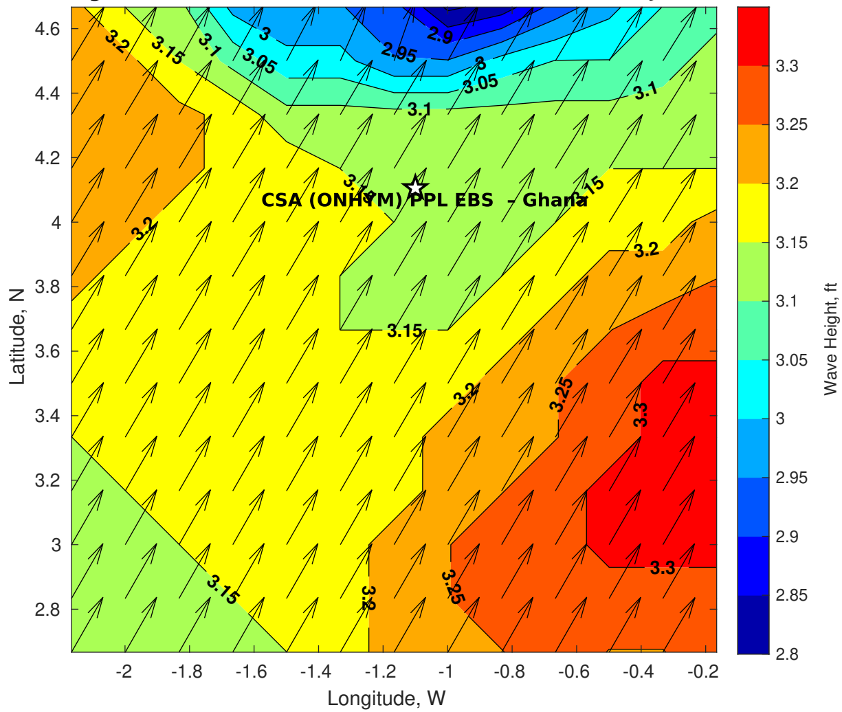
GFS Wave Height (ft) for CSA (ONHYM) PPL EBS - Ghana at 07-Jan-2026 09:00:00
