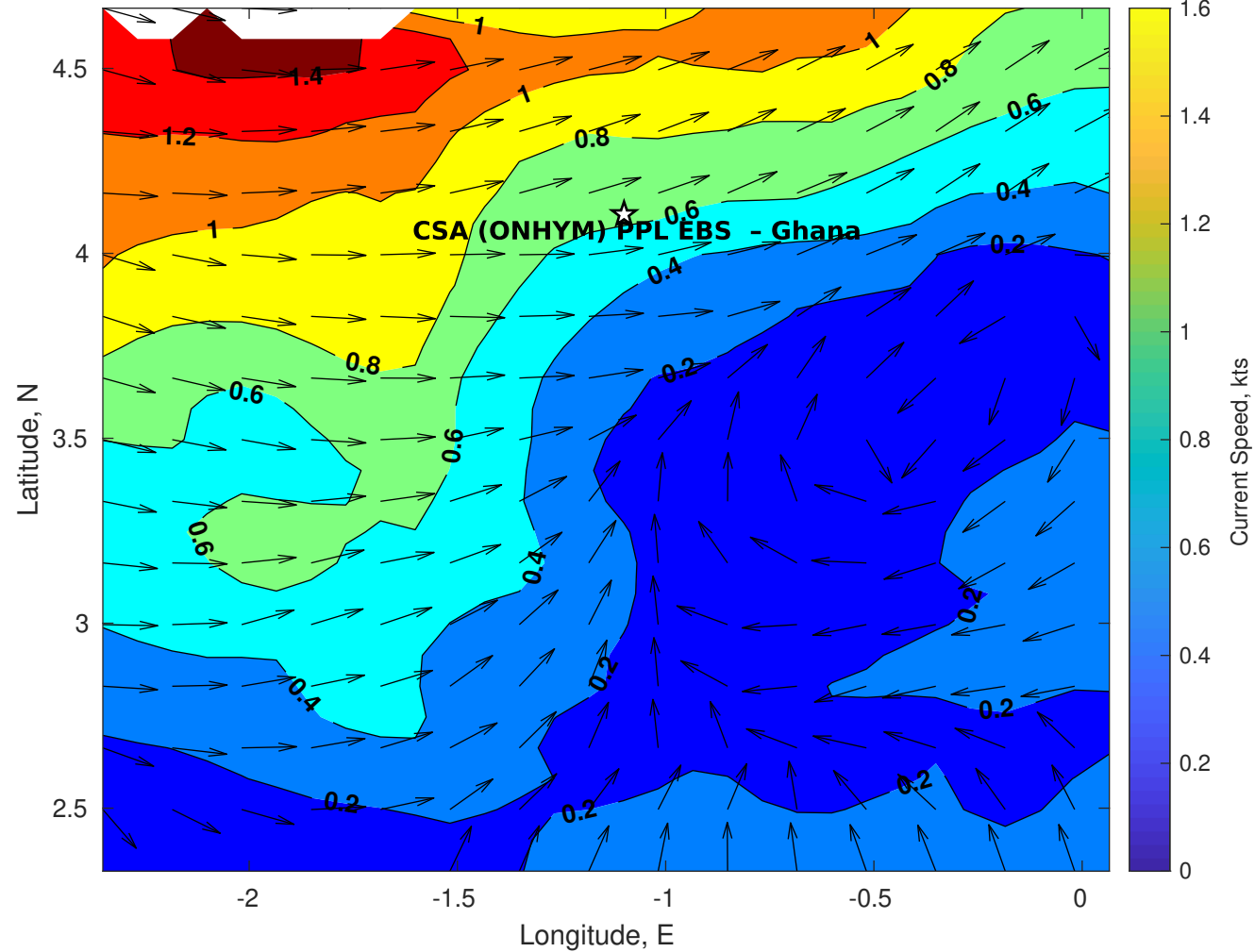
Surface Currents for CSA (ONHYM) PPL EBS - Ghana at 06-Jan-2026 00:00:00
