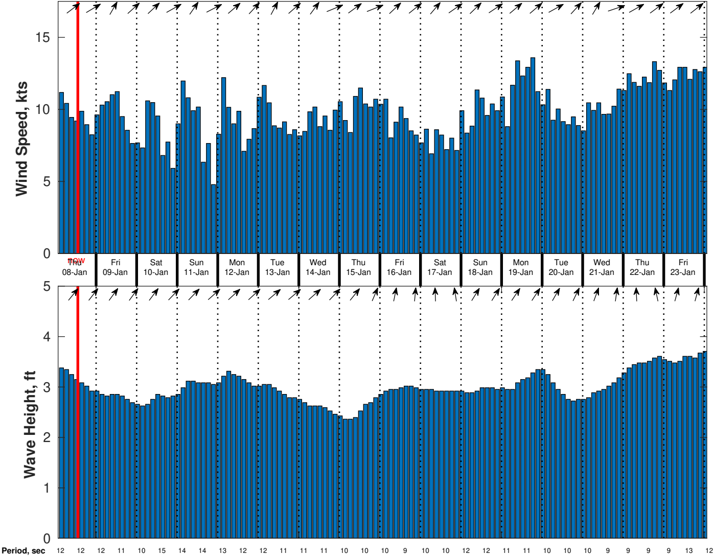
Wind & Wave Forecast for CSA (ONHYM) PPL EBS - Ghana from 07-Jan-2026 02:00:00 to 23-Jan-2026 02:00:00
