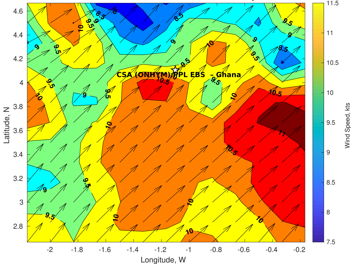
GFS Winds (kts) for CSA (ONHYM) PPL EBS - Ghana at 07-Jan-2026 09:00:00
