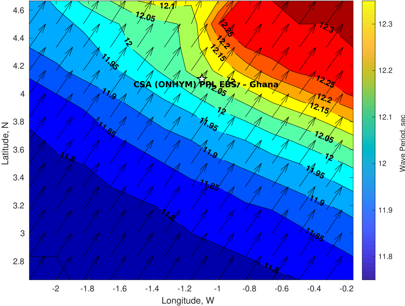
GFS Wave Period (sec) for CSA (ONHYM) PPL EBS - Ghana at 07-Jan-2026 09:00:00
