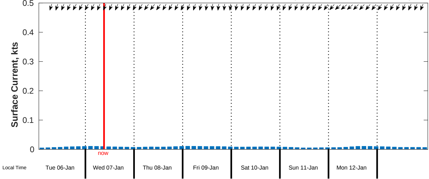
Surface Current Forecast for CSA (ONHYM) PPL EBS - Ghana from 06-Jan-2026 00:00:00 to 14-Jan-2026 00:00:00
