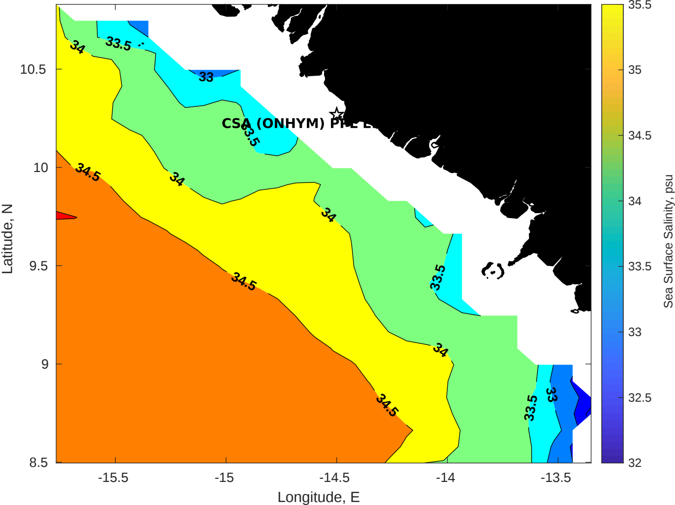
Surface Salinity for CSA (ONHYM) PPL EBS - Guinea at 06-Jan-2026 00:00:00
