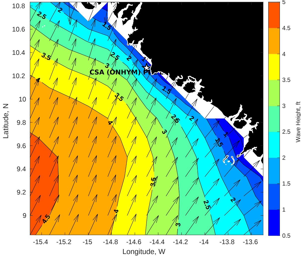
GFS Wave Height (ft) for CSA (ONHYM) PPL EBS - Guinea at 07-Jan-2026 09:00:00
