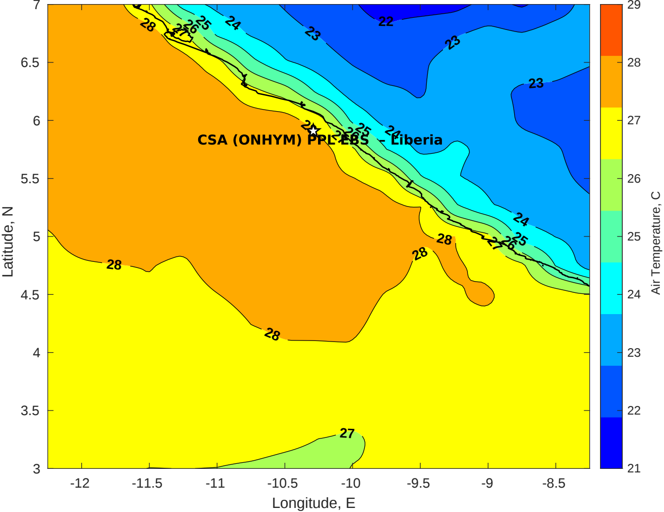
Air Temperature (C) for CSA (ONHYM) PPL EBS - Liberia at 07-Jan-2026
