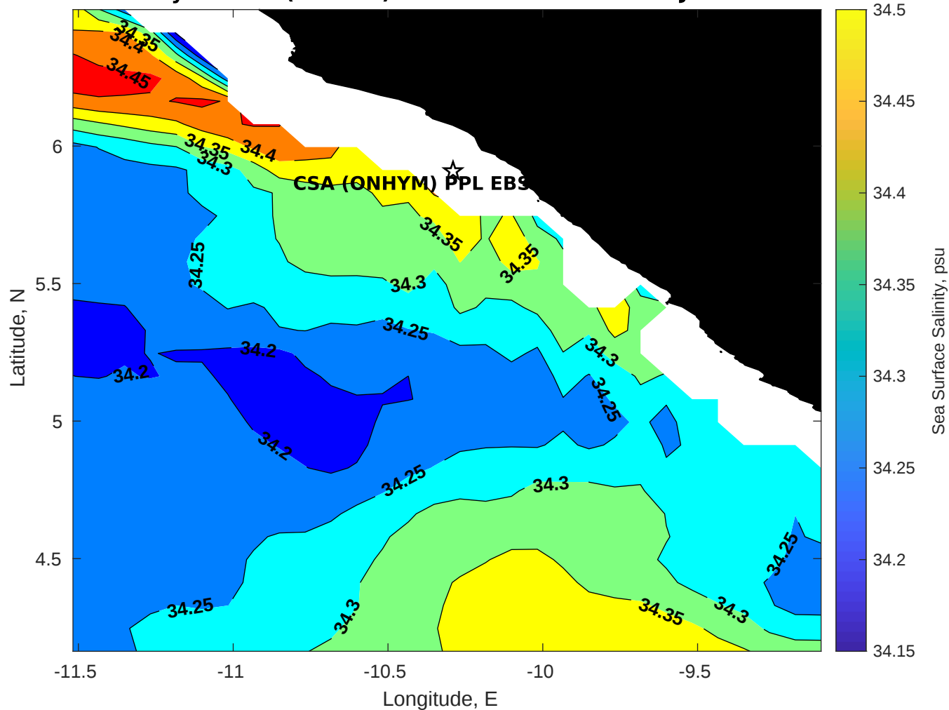
Surface Salinity for CSA (ONHYM) PPL EBS - Liberia at 06-Jan-2026 00:00:00
