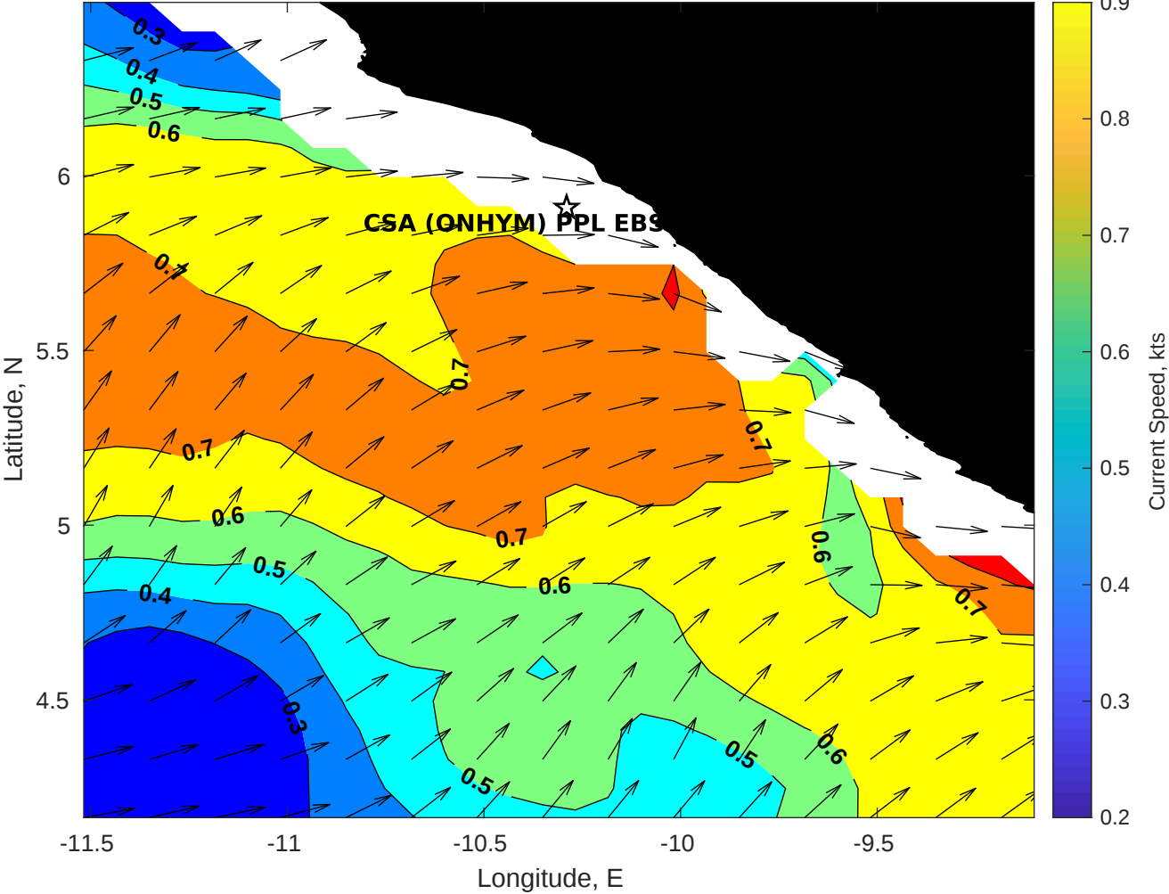
Surface Currents for CSA (ONHYM) PPL EBS - Liberia at 06-Jan-2026 00:00:00
