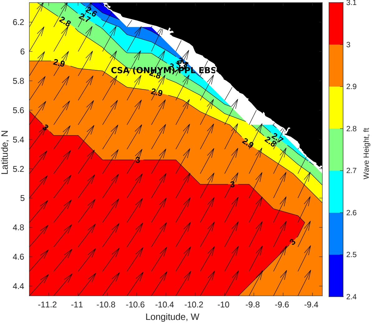
GFS Wave Height (ft) for CSA (ONHYM) PPL EBS - Liberia at 07-Jan-2026 09:00:00
