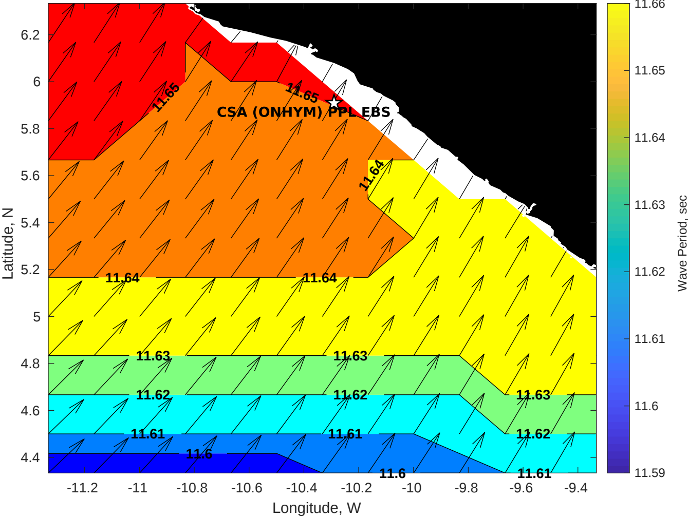
GFS Wave Period (sec) for CSA (ONHYM) PPL EBS - Liberia at 07-Jan-2026 09:00:00
